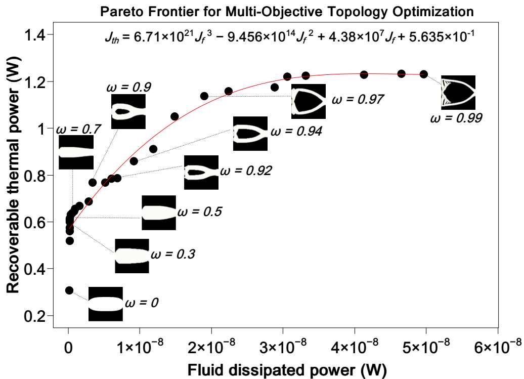
Figure 6: Pareto frontier for multi-objective topology optimization of conjugate heat transfer system.
