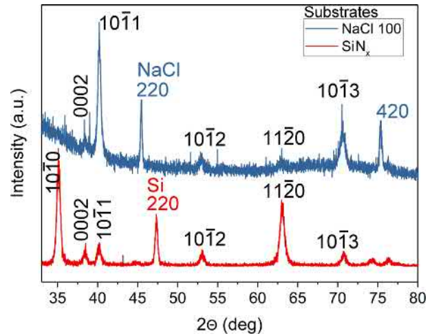
Figure 1: Grazing-Incidence XRD (Cu-K \alpha source) of a 75 nm thick Ti thin film deposited at 200°C on SiN x (100) (sample #Si1) and NaCl (100) (sample #N3). Both films exhibit a polycrystalline microstructure. The film deposited on SiN x shows a strong (10 \bar{1} 0) texture; the film grown on NaCl a (10 \bar{1} 1) texture.
