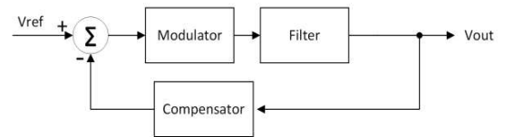
Fig. 4. System control diagram [12]
