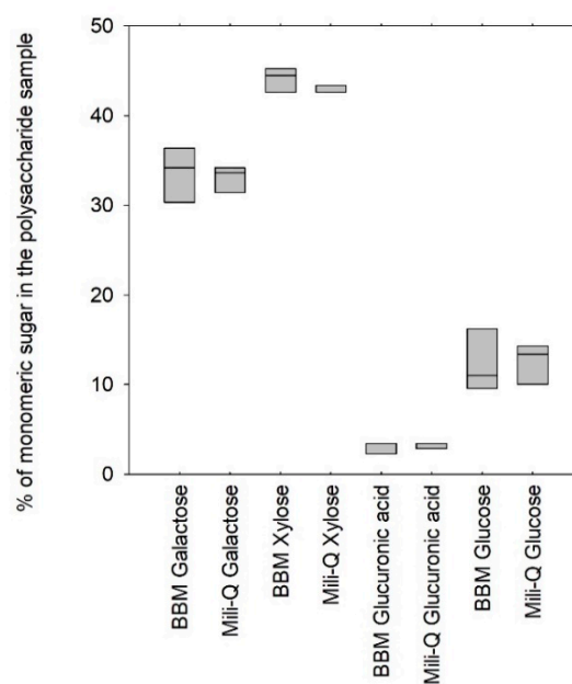
Figure 4. Profile comparison for EPS diluted in Bold's basal medium (BBM) culture medium and milli-Q water prior to hydrolysis.
