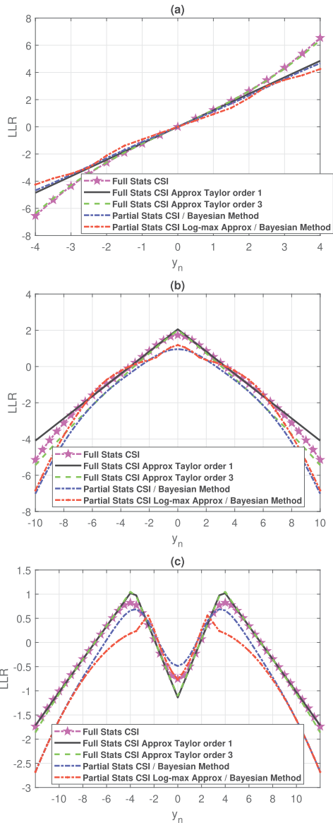
Fig. 1. LLR values \mathcal{L}_n^{(1)} (a), \mathcal{L}_n^{(2)} (b) and \mathcal{L}_n^{(3)} (c) as functions of the channel output y_n for 8-PAM modulation under a normalized Rayleigh channel at SNR = 7.91 dB.
