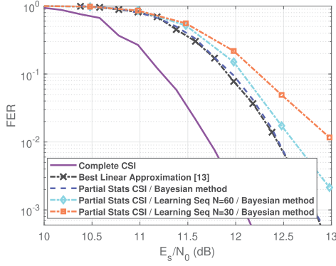
Fig. 4. GPS LIC frame error rate under a Rayleigh channel with a = 0.2 .
