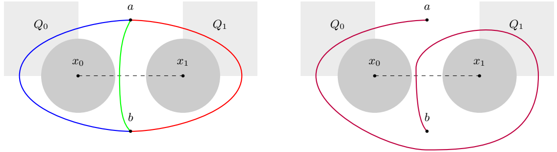
Figure 3: On the left the blue arc belongs to the set H_0 , the green arc to I and the red arc to H_1 . On the right, the purple arc belongs to H_0 , H_1 and I .
