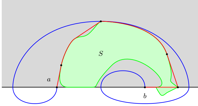
Figure 1: Proposition 2 states that the blue curve with endpoints a and b has a turn greater than the red curve \partial \text{conv}(H_{a,b} \cap S \cup [a, b]) \setminus (a, b) where H_{a,b} is the grey half-plane.
