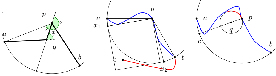
Figure 2: Left: the turn of the polyline [a, q, p, b] , \gamma + \delta , is greater than \alpha + \delta = \pi (the half-line passing through p and q is the bisector of the angle \widehat{apb} ). Center: in blue the arc C_{a,b} = C \cap \bar{B}(p, \frac{\delta}{\sqrt{2}}) . In red, another arc of C whose end c is inside a square having p for vertex and included in the shape bounded by C . Right: in blue, the arc C_{a,b} = C \cap \bar{B}(p, \frac{\delta}{\sqrt{2}}) . The disk \bar{B}(p, d(p, q)) is included in the shape bounded by C . Since the arc C_{a,b} cuts the radius [p, c] passing through q , its turn is greater than that of the quarter of circle in red.
