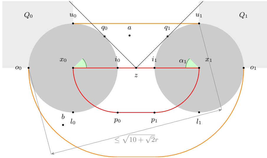
Figure 4: The figure illustrates the notations used in the proof of Lemma 1. The proof consists in showing that one of the two red paths joining the points x_0 x_1 is included in A \ominus \bar{B}(0, r) .
