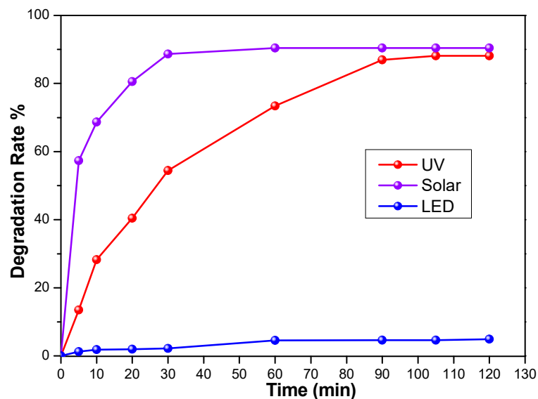
Figure 9. The photocatalytic activity of \text{ZnBi}_2\text{O}_4 under UV, sunlight and LED lamp: CCFX = 10 ppm, pH ~6, T = 25 \text{ }^\circ\text{C} and catalyst dose = 1 g/L.
