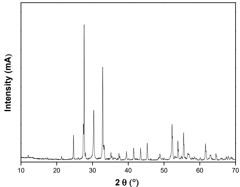
Figure 1. XRD diffractogram of ZnBi_2O_4 calcined at 600 °C.
