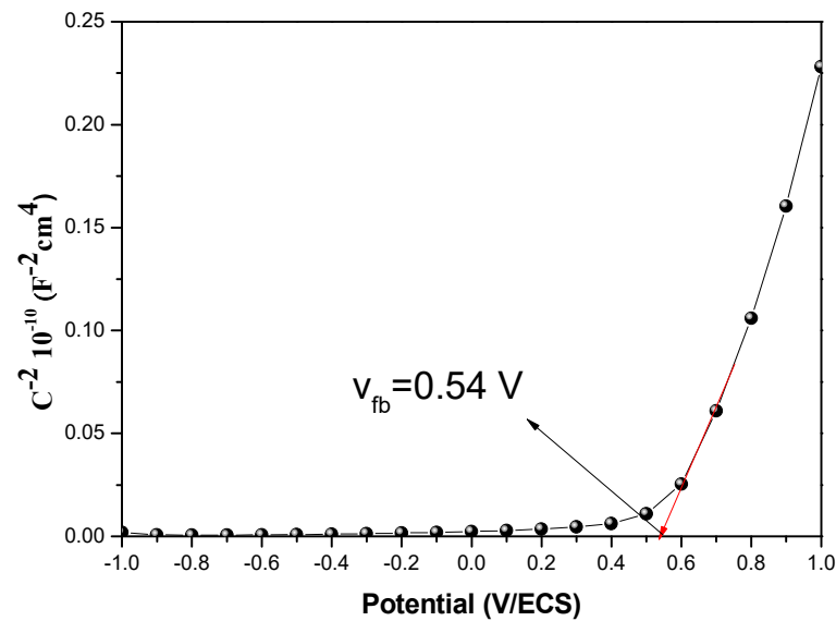
Figure 7. The capacitance-potential characteristic of \text{ZnBi}_2\text{O}_4 in \text{NaOH} (0.1 M) solution.
