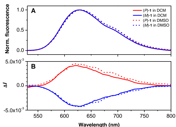
Figure 6. (A) Emission and (B) CPL spectra of ( P )- 1 (in red) and ( M )- 1 (in blue). The measurements were performed in DCM (solid lines) or DMSO (dashed lines) for both panels.
