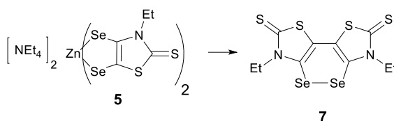
Scheme 6 Synthesis of diselenine 7 from the proligand 5 . Reagents and conditions : electrocrystallization
