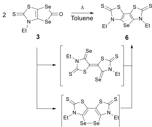
Scheme 3 Synthesis of selenophene 6 through thermal treatment of 3
