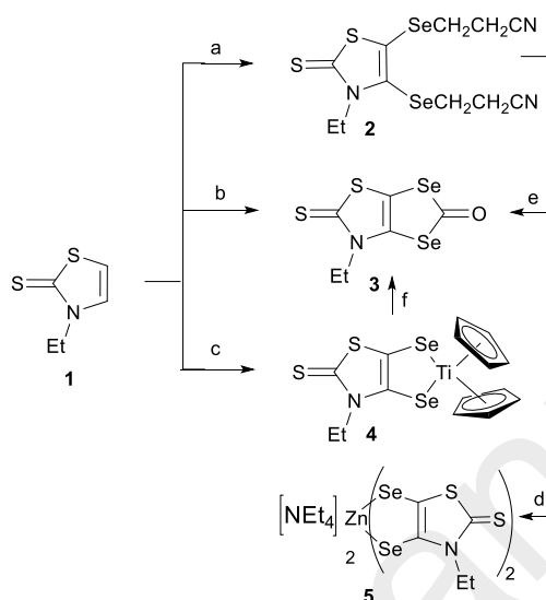
Scheme 2 Synthesis of the different diselenolene proligands 2-5 . Reagents and conditions: (a) LDA, Se, BrCH 2 CH 2 CN, (b) LDA, Se (Cl 3 CO) 2 CO, (c) LDA, Se, Cp 2 TiCl 2 , (d) MeONa, ZnCl 2 , NEt 4 Br. Alternative routes to 3 from proligands 2 and 4 . Reagents and conditions: (e) LDA, (Cl 3 CO) 2 CO, (f) (Cl 3 CO) 2 CO, THF, Δ.
