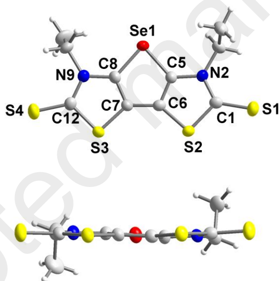
Fig. 1 Molecular structure of selenophene 6 (top) and side view (bottom). Thermal ellipsoids are drawn at the 80 % probability level.
