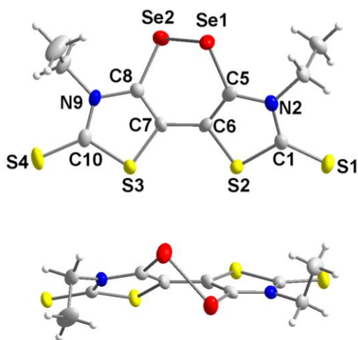
Fig. 2 Molecular structure (top) and side view (bottom) of diselenine 7 . Ellipsoids are drawn at 80 % probability.
