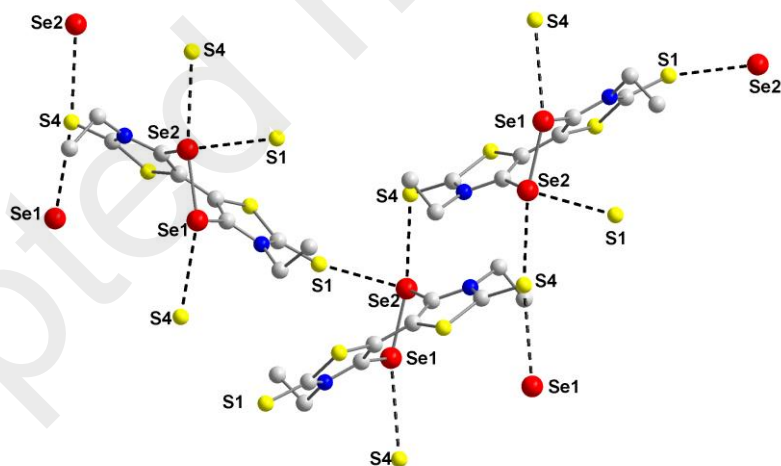
Fig. 3 Details of the shortest Se...S interaction network in 7
