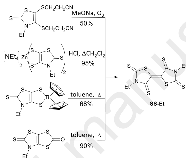
Scheme 1 Comparison of the efficiency of the different synthetic routes towards SS-Et starting from different various proligands
