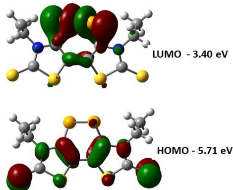
Fig. 5 HOMO and LUMO of diselenine 7 shown with a cut-off of 0.04 \text{ [e/bohr}^3]^{1/2} .
