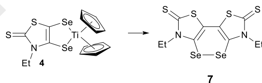
Scheme 5 Synthesis of diselenine 7 from the proligand 4 . Reagents and conditions : NaCl, CH 2 Cl 2 /THF, 35°C for 4 days.
