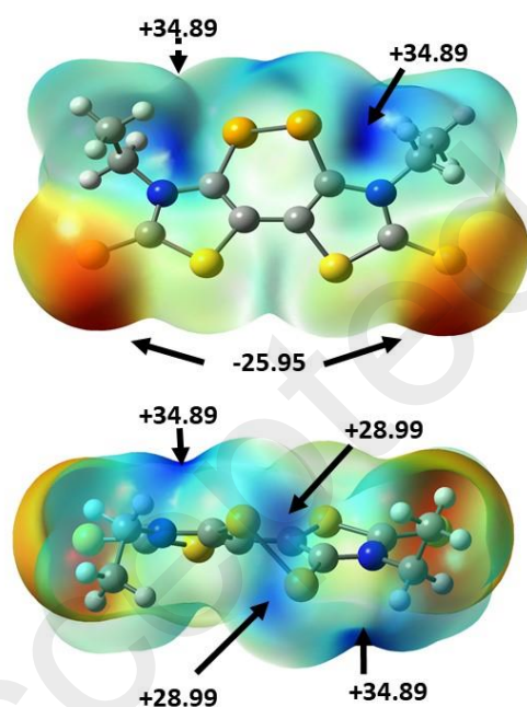
Fig. 4 Molecular electrostatic potential surfaces mapped at 0.001 \text{ e}^-.\text{au}^{-3} isodensity surface for 7 . The common color scale ranges from -26 \text{ kcal.mol}^{-1} (red) to +35 \text{ kcal.mol}^{-1} (blue).
