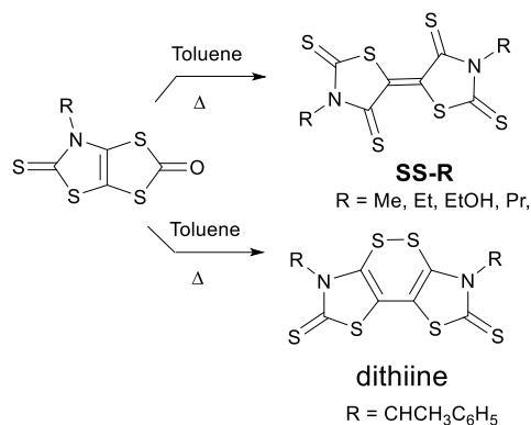
Scheme 4 Synthesis of either SS-R or dithiine
