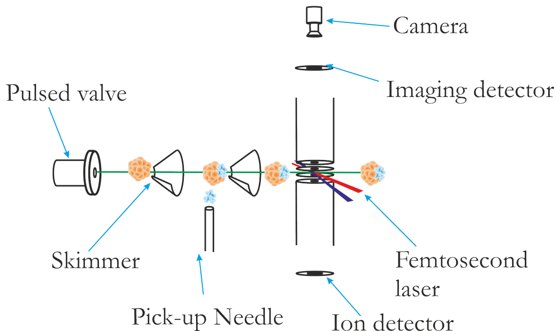
Figure 2: Experimental Setup.
