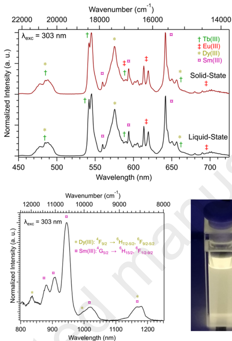
Figure 6. Emission spectra ( \lambda_{exc} = 303 nm) of [\text{Sm}_{0.07}\text{Eu}_{0.02}\text{Tb}_{0.04}\text{Dy}_{0.07}\text{La}_{1.8}(\text{dcpa})_3(\text{H}_2\text{O})]_{\infty} and [\text{Sm}_{0.07}\text{Eu}_{0.02}\text{Tb}_{0.04}\text{Dy}_{0.07}\text{La}_{1.8}(\text{dcpa})_3(\text{H}_2\text{O})]_{\infty}:\text{EtOH} ( 0.3 \text{ g}\cdot\text{L}^{-1} ) in the visible domain (top) and of [\text{Sm}_{0.07}\text{Eu}_{0.02}\text{Tb}_{0.04}\text{Dy}_{0.07}\text{La}_{1.8}(\text{dcpa})_3(\text{H}_2\text{O})]_{\infty}:\text{EtOH} ( 0.3 \text{ g}\cdot\text{L}^{-1} ) in the IR domain (bottom left). Picture under UV irradiation of a [\text{Sm}_{0.07}\text{Eu}_{0.02}\text{Tb}_{0.04}\text{Dy}_{0.07}\text{La}_{1.8}(\text{dcpa})_3(\text{H}_2\text{O})]_{\infty}:\text{EtOH} ( 0.3 \text{ g}\cdot\text{L}^{-1} ; \lambda_{exc} = 312 nm) suspension (bottom right).
