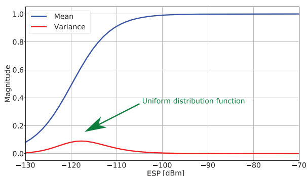
FIGURE 7 Mean \mathbb{E}[PDR] and variance Var[PDR] evolution against ESP
