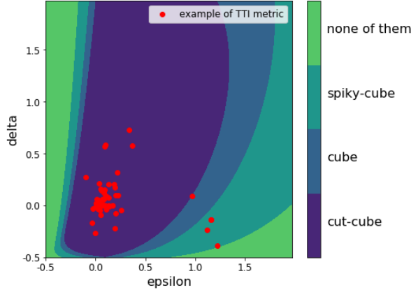
Figure 2: Acuteness property for TTI metrics. The figure shows whether a given stencil is acute with respect to a TTI metric determined by Thomsen parameters (\epsilon, \delta) , with V_p = 1 and V_s = 0 , while taking into account the worst possible rotation of the metric. The domain labelled for the spiky-cube also contains the domain labelled for the cube, which also contains the domain labelled for the cut-cube.
