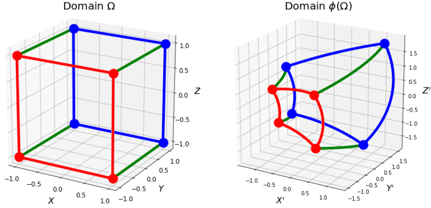
Figure 3: Edges of the domain \tilde{\Omega} = ]-1, 1[^3 (a cube) and of its image \Omega = \phi(\tilde{\Omega}) by the special conformal transformation (40). See §4.1 and §A.
