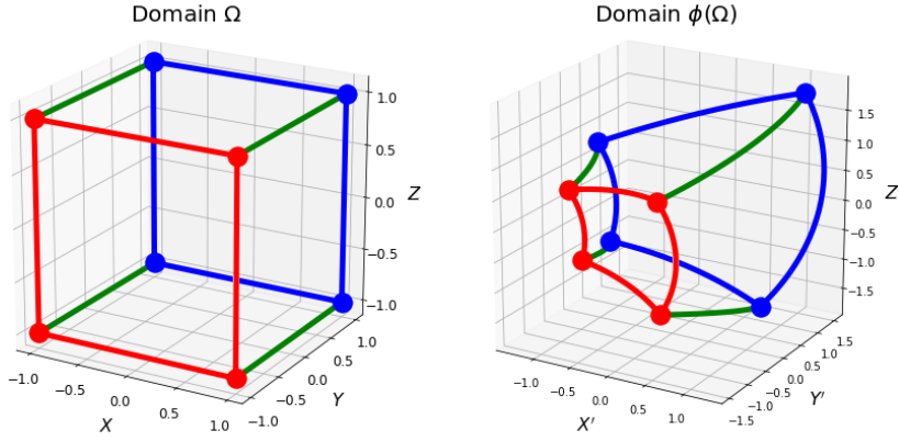
Fig. 3 Edges of the domain \tilde{\Omega} = ]-1, 1[^3 (a cube) and of its image \Omega = \phi(\tilde{\Omega}) by the special conformal transformation (40). See §4.1 and §A.
