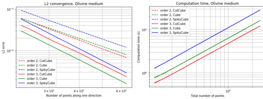
Fig. 5 Convergence orders for the olivine, comparison between stencils
