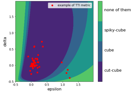
Fig. 2 Acuteness property for TTI metrics. The figure shows whether a given stencil is acute with respect to a TTI metric determined by Thomsen parameters (\epsilon, \delta) , with V_p = 1 and V_s = 0 , while taking into account the worst possible rotation of the metric. The domain labelled for the spiky-cube also contains the domain labelled for the cube, which also contains the domain labelled for the cut-cube.
