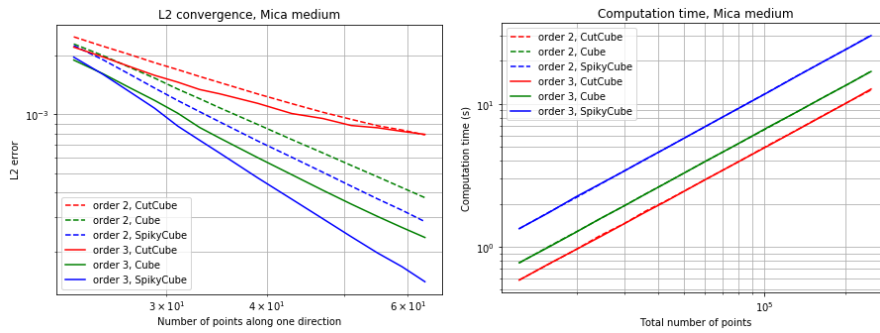
Fig. 6 Convergence orders for the mica, comparison between stencils
