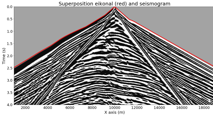
Fig. 8 Seismogram recorded along a receiver line located on the surface ( z = 0 km), in the source plane ( y = 10 km) along the x -axis (from x = 0 km to x = 20 km). The vertical displacement is recorded. The vertical displacement intensity is represented in black and white. The first-arrival travel-time computed through our eikonal solver for each receiver position is superposed to the seismogram in red. The resulting red-contour matches the synthetic first-arrival travel-time corresponding to the 3D spectral-element simulation.
