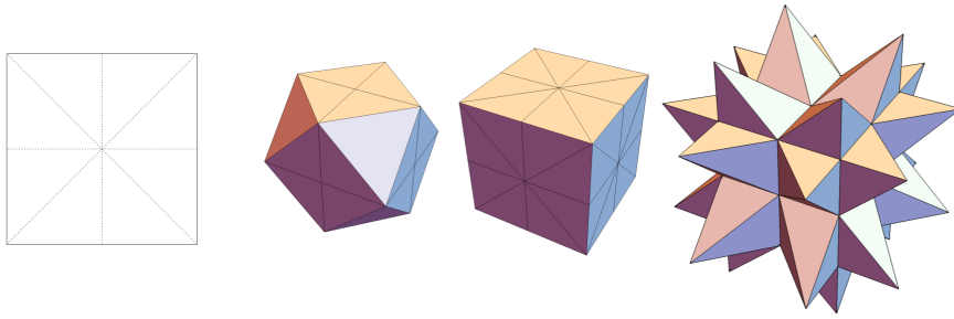
Fig. 1 Stencils used, in dimension 2 (square) and 3 (cut-cube, cube and spiky-cube)
