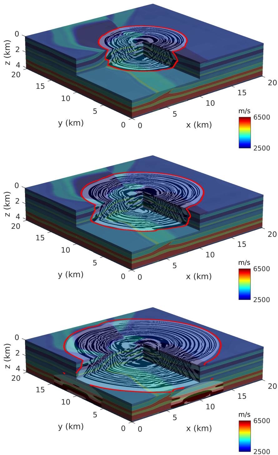
Fig. 7 Elastic wavefield (black and white) computed in the 3D fully anisotropic medium coming from the homogenization of the SEG/EAGE overthrust model. The background corresponds to \sqrt{\frac{C_{33}}{\rho}} , that is the P-wave velocity of this model if it had a VTI symmetry (which is not the case here, but it still gives a good approximation for illustrative purposes). The red contour corresponds to the isochrone computing through our fast marching eikonal solver. The different snapshots are obtained at t = 1.5 s (top), t = 2 s (middle) and t = 2.5 s (bottom).
