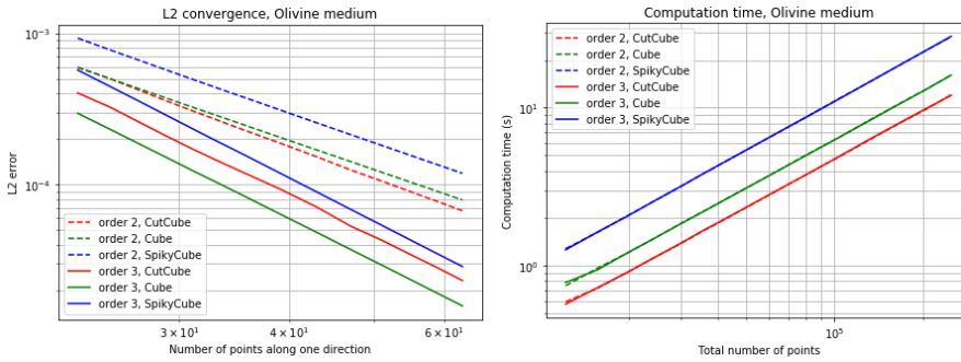
Fig. 5 Convergence orders for the olivine, comparison between stencils
