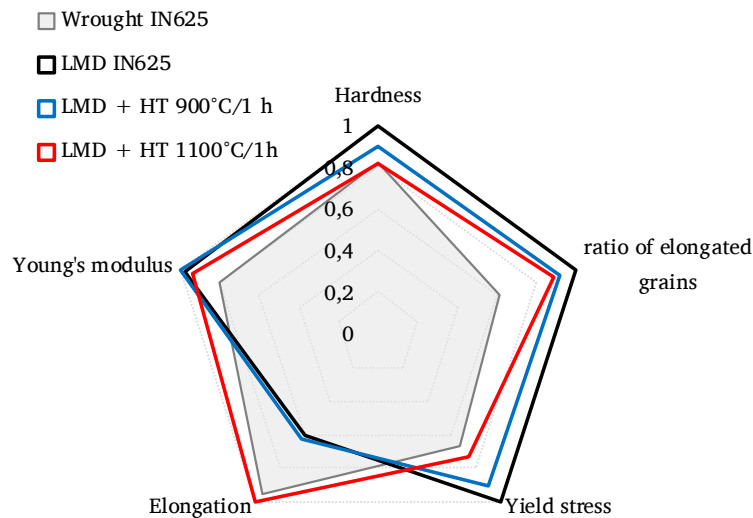
Figure 19: Effect of post-annealing treatments on the microstructure and mechanical properties of LMD samples.
