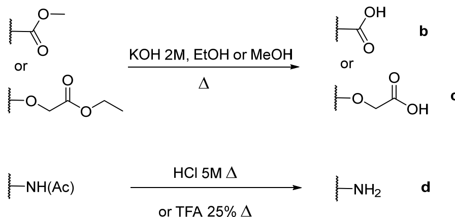
Figure 1. Deprotection of carboxylic acid and amine functions.
