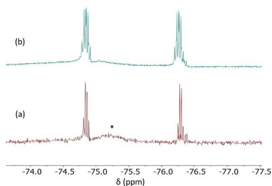
Figure 4. ^{19}\text{F}\{^1\text{H}\} NMR (a) and ^{19}\text{F} NMR (b) spectrum of 4 in \text{CDCl}_3 .
