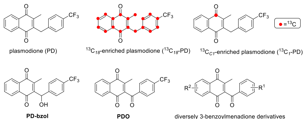
Figure 1. Structures of the chemical tools investigated in this study: the antimalarial plasmodione (PD) and both ^{13}\text{C}_{18/7} -enriched representatives ( ^{13}\text{C}_{18} -PD and ^{13}\text{C}_7 -PD), its two metabolites (PD-bzol and PDO), and diversely substituted 3-benzoylmenadiones.
