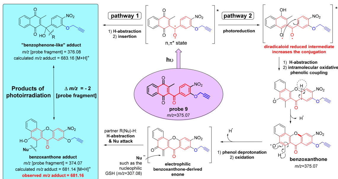
Scheme 2. Chemical Analysis of the Insertion Products upon Photoirradiation of the ABPP Probe 9 with Glutathione (GSH) by Mass Spectrometry a
