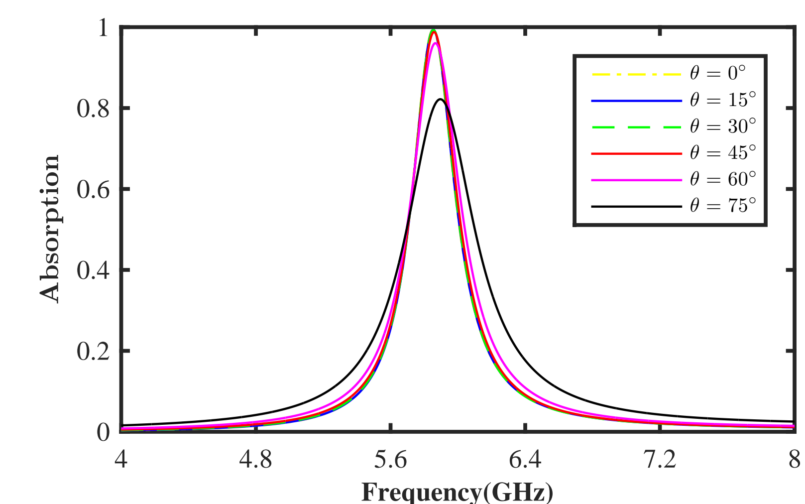
Figure 9: Absorption as a function of \theta ( \phi = 0^\circ )
