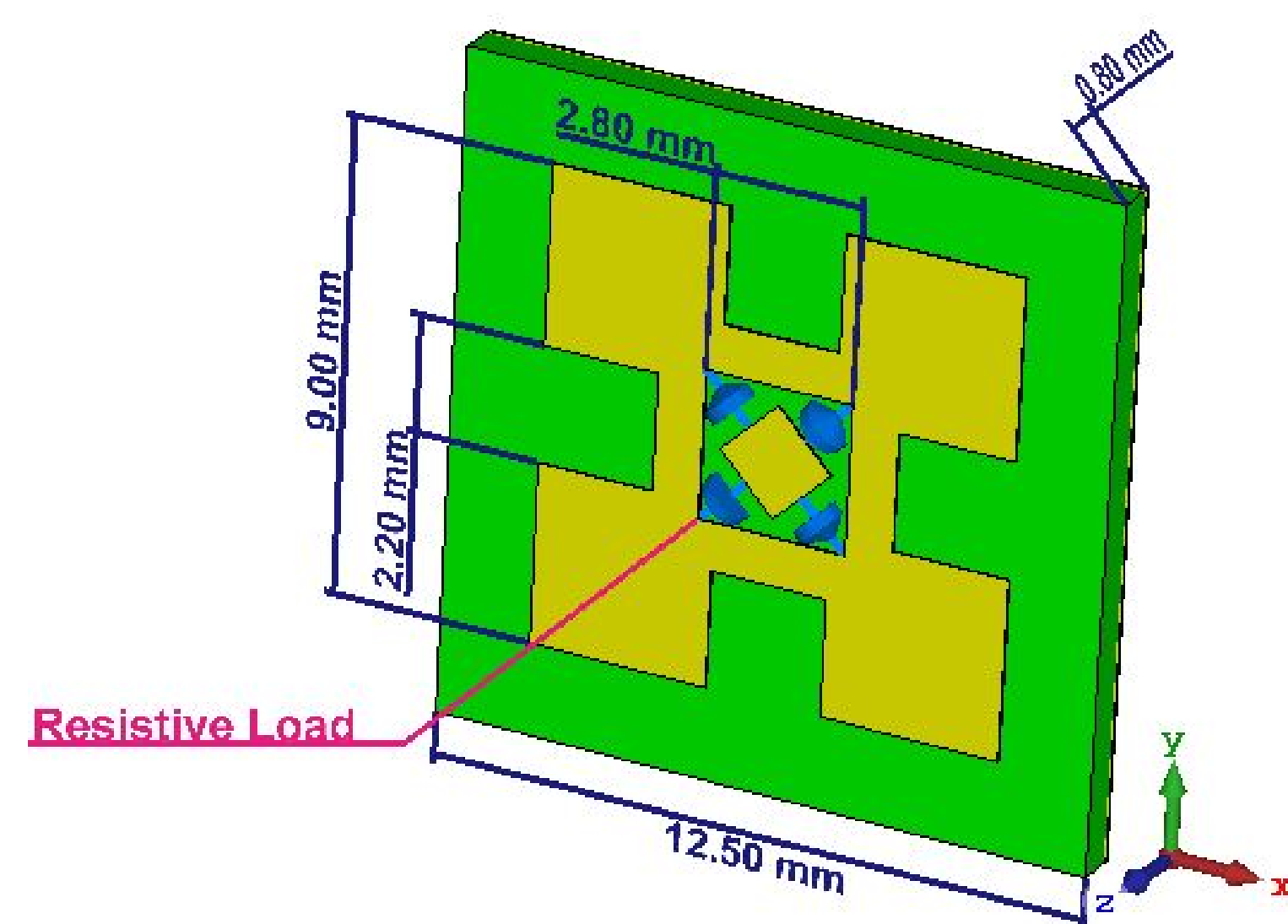
Figure 1: Unit-Cell Geometry
