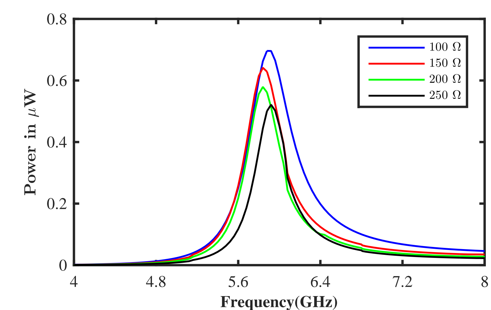
Figure 11: AC power as a function of frequency
