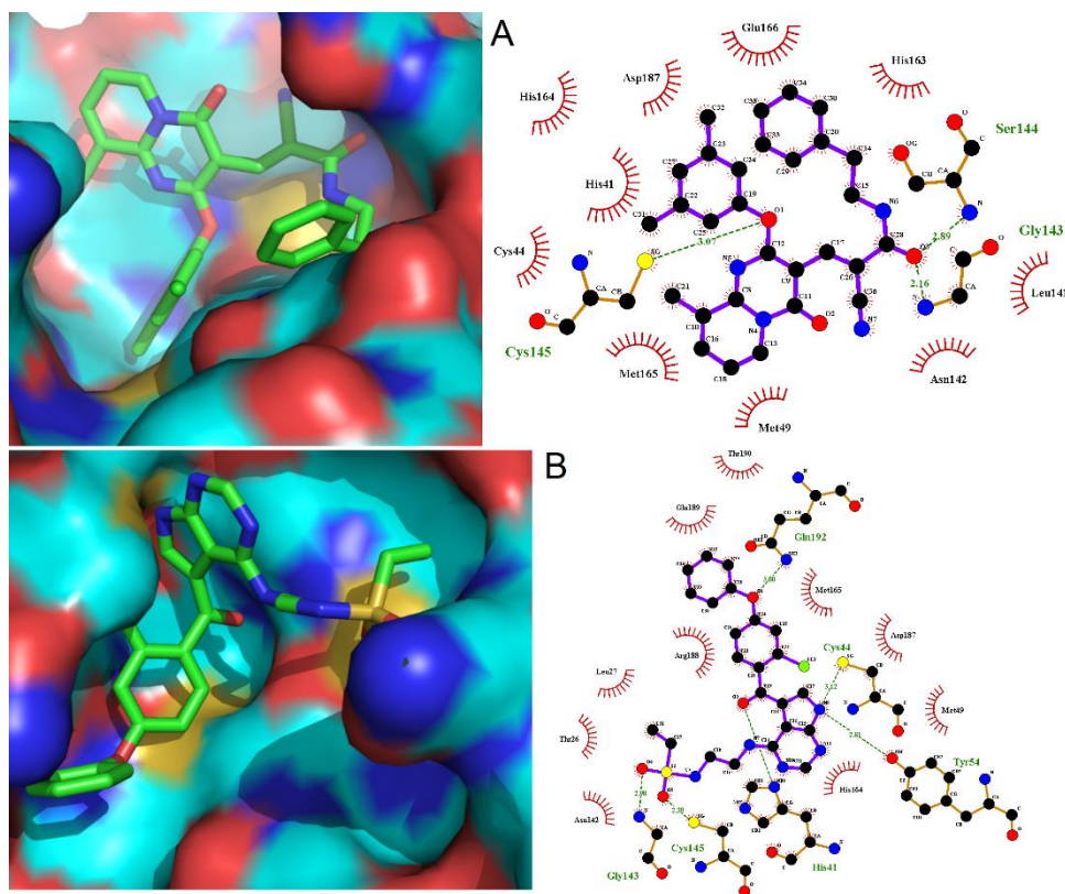
Figure 5. Binding modes of compounds 2011299 (A) and 134294169 (B) with the corresponding hydrogen bonds network.
