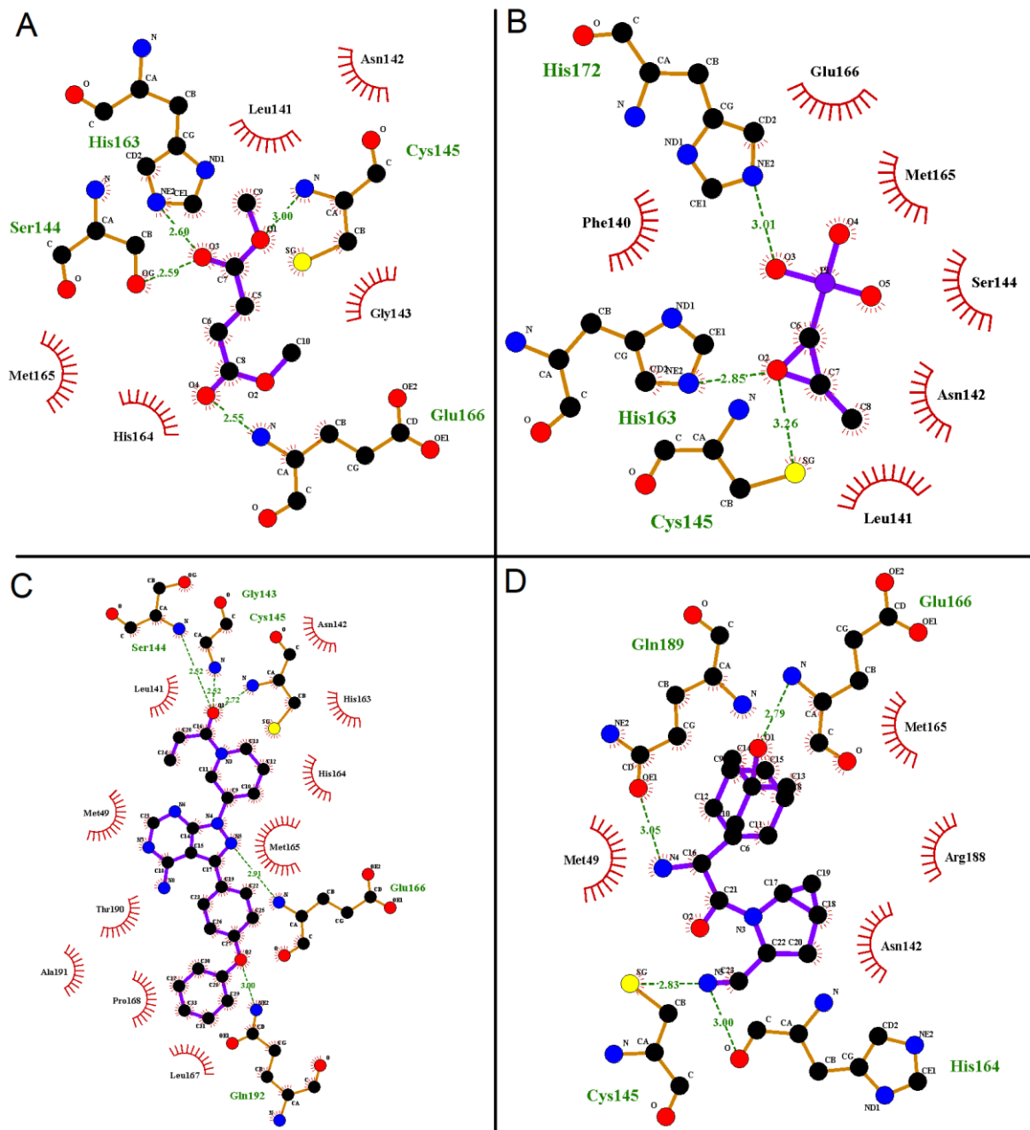
Figure 6. 2D representation of the proposed binding modes of the four potential covalent inhibitors within the binding site of M^{Pro} : dimethylfumarate (A), fosfomycin (B), ibrutinib (C), saxagliptin (D).
