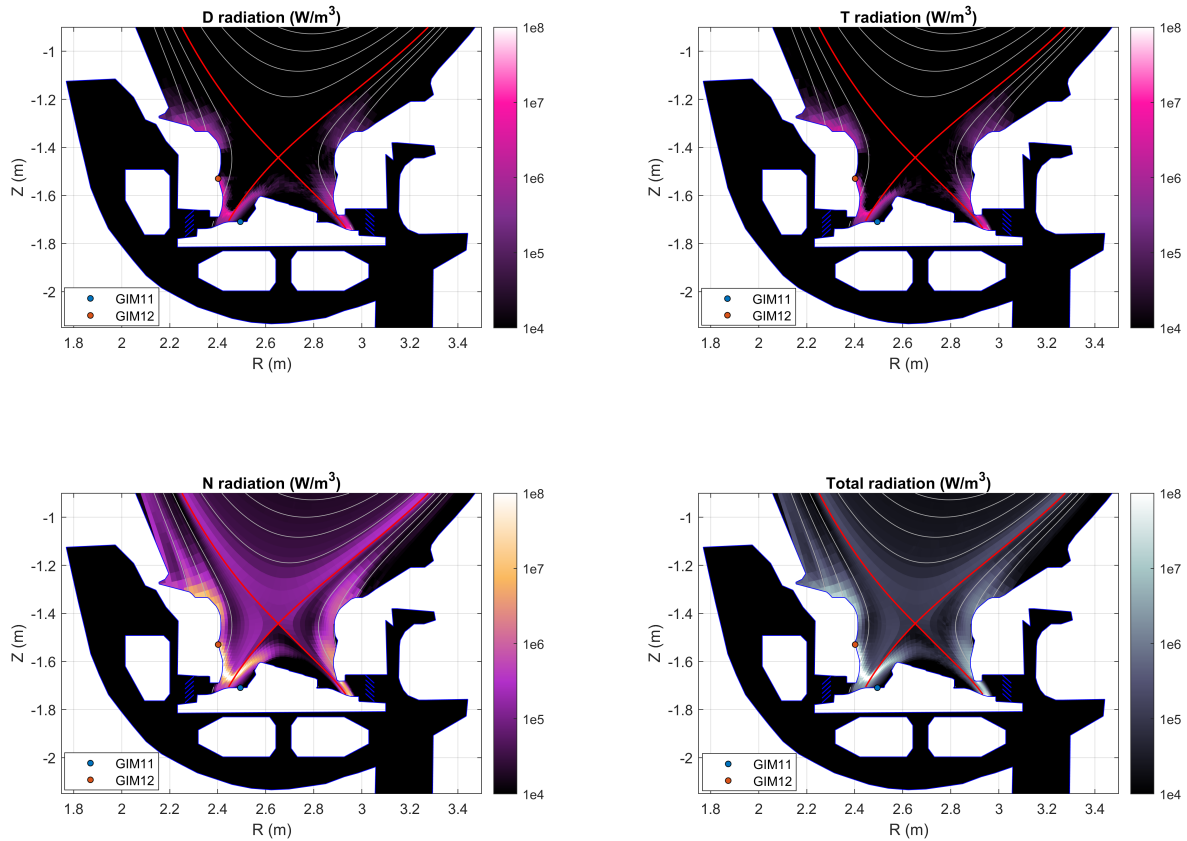
Figure 12. 2D maps of radiation for the different species.
