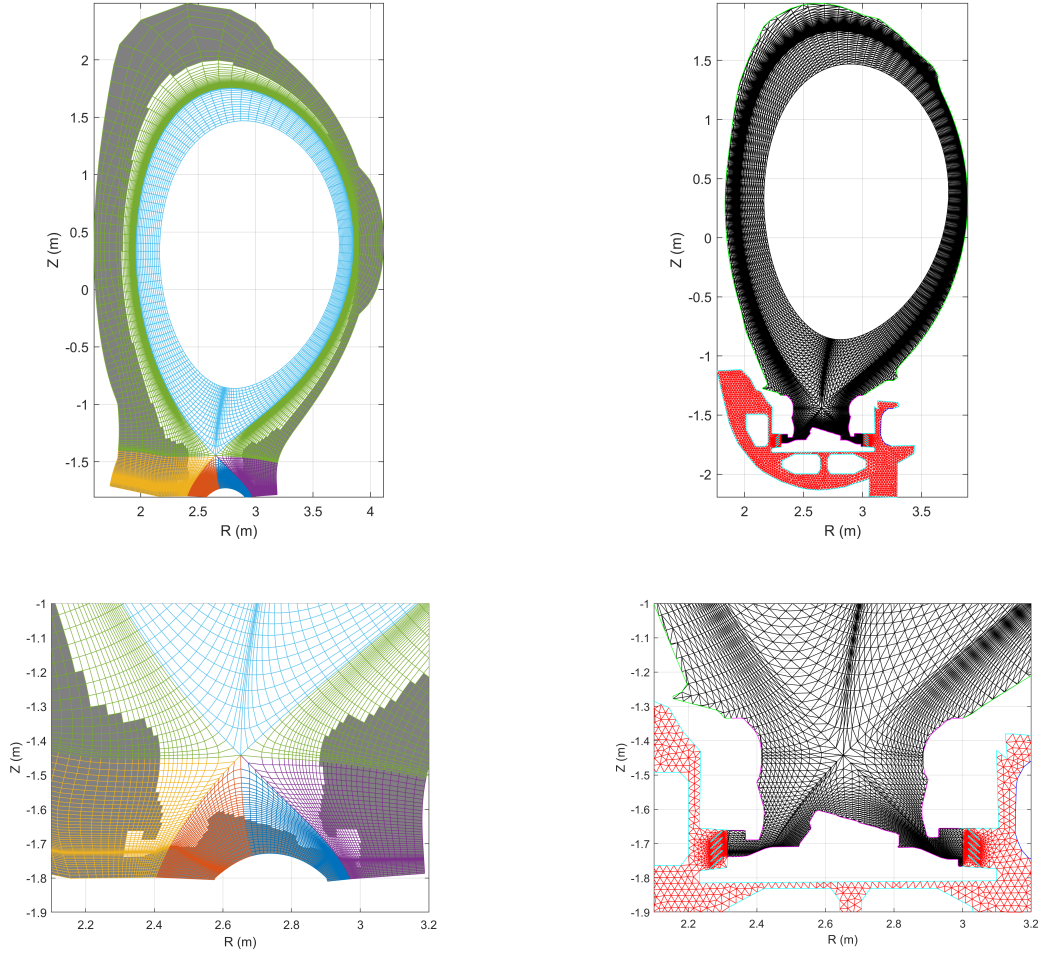
Figure 6. Soledge2D-EIRENE mesh based on JET #97395 equilibrium at t = 50 s. Left: Soledge2D mesh based on quadrangles grid extended to the wall. Right: EIRENE grid based on triangles. Wall types are identified with different colors (green for Be, blue for W and red for pumping surfaces). Gas Puffs are identified by triangle symbols (Orange GIM4 and Violet GIM10).
