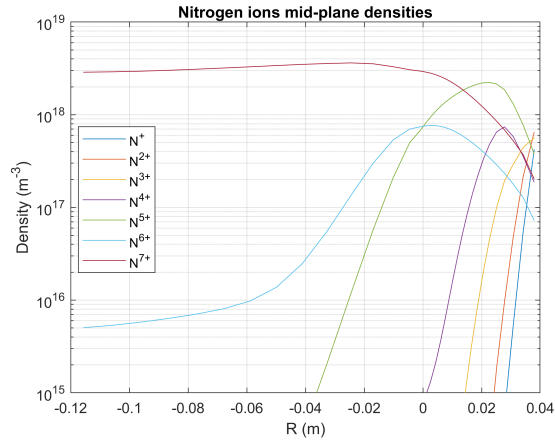
Figure 11. Radial profiles of plasma ion species at the outer midplane.
