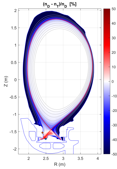
Figure 10. Relative difference between deuterium and tritium density
