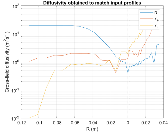
Figure 7. Transport coefficients used in JET D-T simulation. radial dependency at the LFS midplane.
