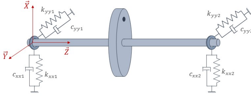
Figure 3: rotor exemple
