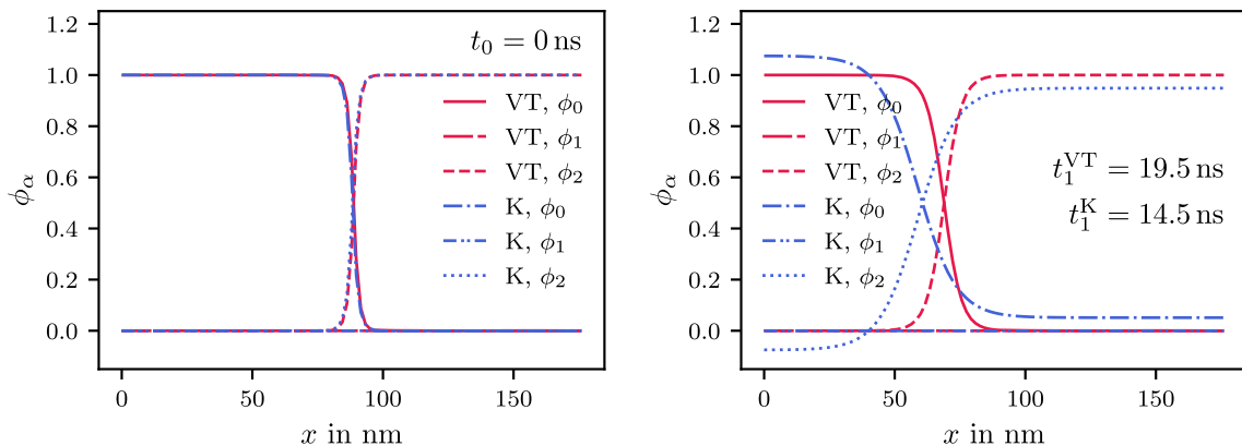
Fig. 7 Phase field for the parent phase \phi_0 (solid, dash-dot), and the martensitic orientation variants \phi_1 (dashes, dash-dot-dot) and \phi_2 (small dashes, dots) for the Khachaturyan using a linear interpolation (K, blue) and the Voigt/Taylor approach using a cubic interpolation (VT, red). The solution at t_0 is shown on the left, and the stable state after evolution is shown on the right (color figure online)
