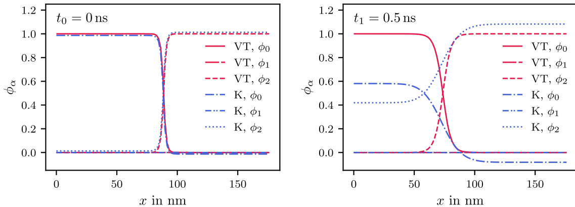
Fig. 6 Phase field for the parent phase \phi_0 (solid, dash-dot), and the martensitic orientation variants \phi_1 (dashes, dash-dot-dot) and \phi_2 (small dashes, dots) for the Khachaturyan using a linear interpolation (K, blue) and the Voigt/Taylor approach using a cubic interpolation (VT, red). The solution at t_0 is shown on the left, and the evolution after t_1 = 0.5 ns on the right
