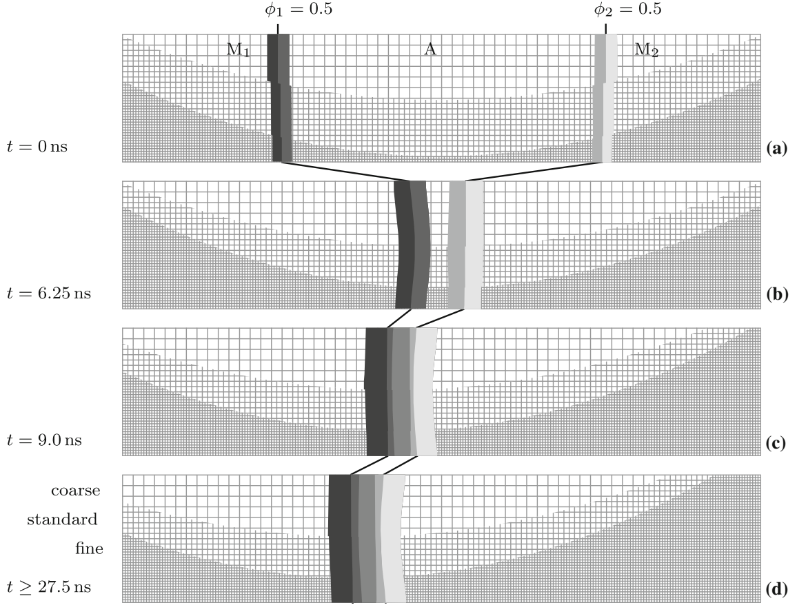
Fig. 3 Time evolution of the martensitic transformation for different levels of mesh refinement. The solid colored regions indicate the interface region where 0.2 < \phi_1 < 0.8 (left, dark grey), and where 0.2 < \phi_2 < 0.8 (right, light grey). Initially, the austenitic phase is present in the center (A), with the martensitic orientation variants to the left ( M_1 ) and right ( M_2 )
