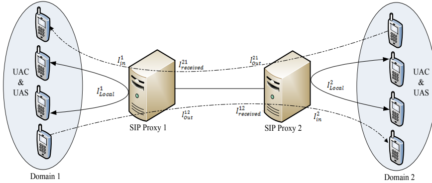
Figure 2: SIP network with two servers
