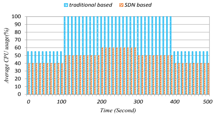
Figure 15: The average CPU usage of servers over time
