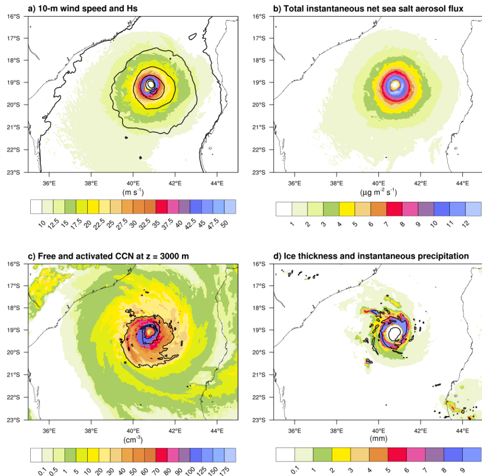
Figure 5. Horizontal cross sections of Idai on 12 March 2019 at 18 UTC, simulated with the Meso-NH/WW3/CROCO OWA coupled system. (a) 10-m wind speed (m s -1 ; colors) and significant wave height H_s (2, 4, 6, 8 and 10 m isolines), (b) total instantaneous net sea salt aerosol flux ( \mu\text{g m}^{-2} \text{s}^{-1} ), (c) available (colors) and activated (1 and 10 cm -3 isolines) CCN, and (d) total ice thickness (mm; colors) and instantaneous precipitation (10 mm h -1 isoline). In c) only the contribution of sea salt particles (with dry diameter higher than 80 nm) to CCN is shown.
