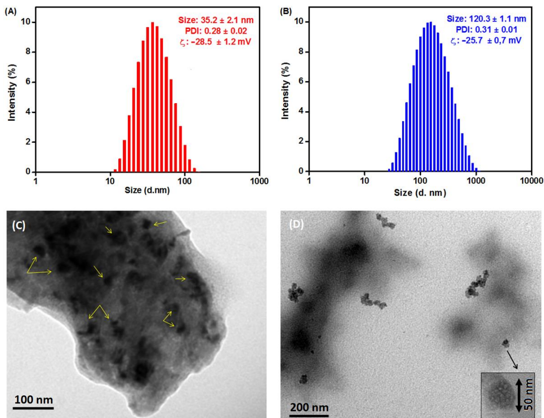
Figure 3. DLS profiles in water of (A) \beta -CD@Cur 4 and (B) (\beta\text{-CD})_2 @Cur 5. TEM images of (C) \beta -CD@Cur 4 and (D) (\beta\text{-CD})_2 @Cur 5.
