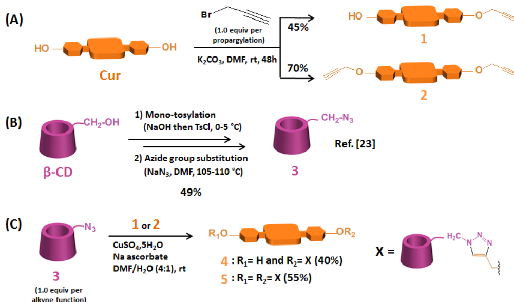
Scheme 1. Synthesis of (A) Cur mono-alkyne 1 and Cur di-alkyne 2, (B) mono-6-azido- \beta -CD 3, and (C) \beta -CD@Cur 4 and (\beta -CD) 2 @Cur 5 nanoconjugates.
