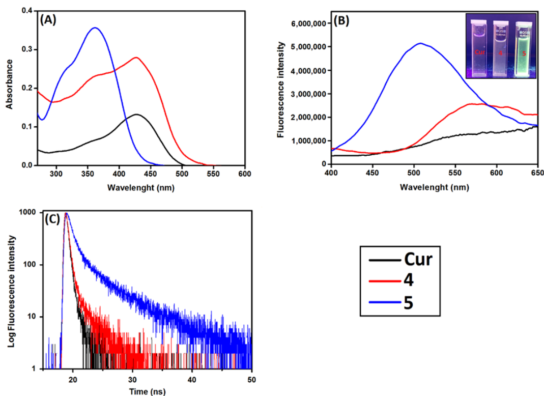
Figure 4. Photophysical properties of Cur, \beta -CD@Cur 4 and (\beta -CD) 2 @Cur 5 in D 2 O at room temperature. (A) UV-vis absorption spectra at a single concentration of Cur ( c = 12 \mu\text{M} ), and (B) fluorescence emission and (C) fluorescence lifetime spectra at \lambda_{\text{exc}} = 360 \text{ nm} ( A_{360 \text{ nm}} = 0.2 ).
