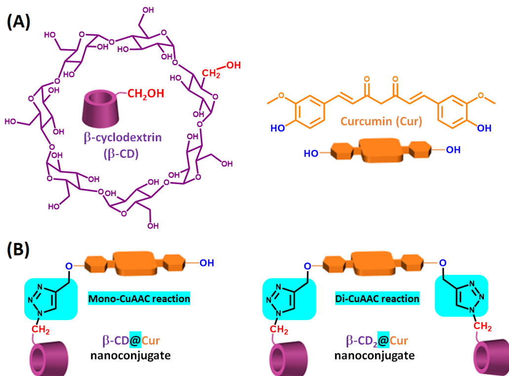
Figure 1. (A) Chemical structures of \beta -CD and Cur, and (B) schematic illustration of \beta -CD@Cur and (\beta -CD) 2 @Cur nanoconjugates obtained through mono- and di-CuAAC reaction.
