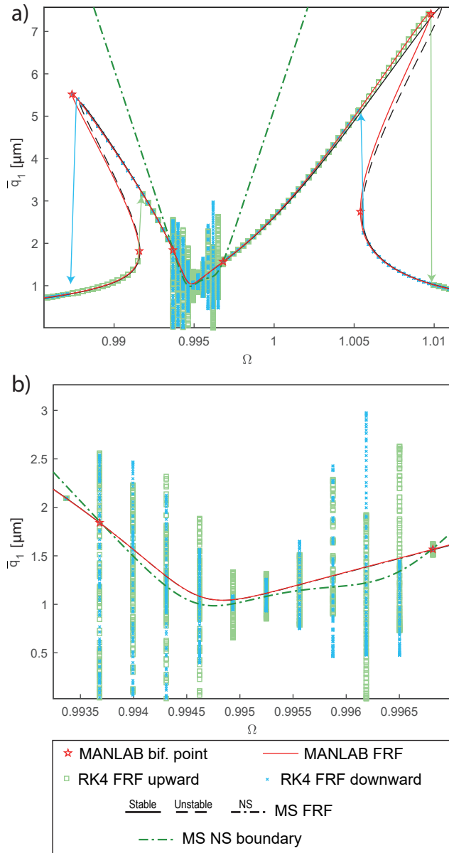
Fig. 17 Detuned condition \omega_2 = 1.989\omega_1 . Comparison between the analytical solution from Eqs. (27) (black line), continuation of periodic orbits of Eqs. (1) (red lines) and the time-marching integration of Eqs. (1) (circle markers). The analytical NS boundary is the green dash-dotted line. The red star markers define the bifurcation points identified by MANLAB.
