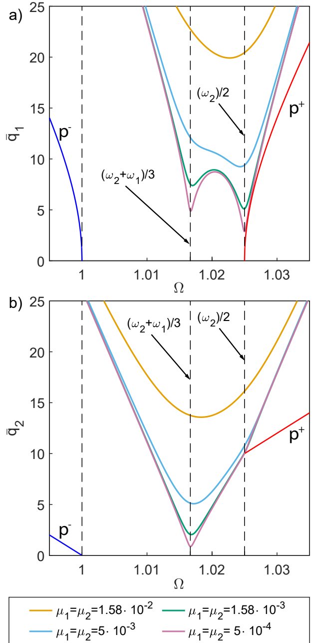
Fig. 10 Behaviour of the NS boundary curve, for \omega_1 = 1 , \omega_2 = 2.05 , \alpha_{12} = 1 \cdot 10^{-2} , \alpha_{11} = 5 \cdot 10^{-3} and different values of \mu_1 = \mu_2 as detailed in the legend. The blue and red continuous lines are the backbone of the p^- and p^+ mode while the black dashed lines correspond to \Omega = \omega_2/2 and \Omega = (\omega_1 + \omega_2)/3 .
