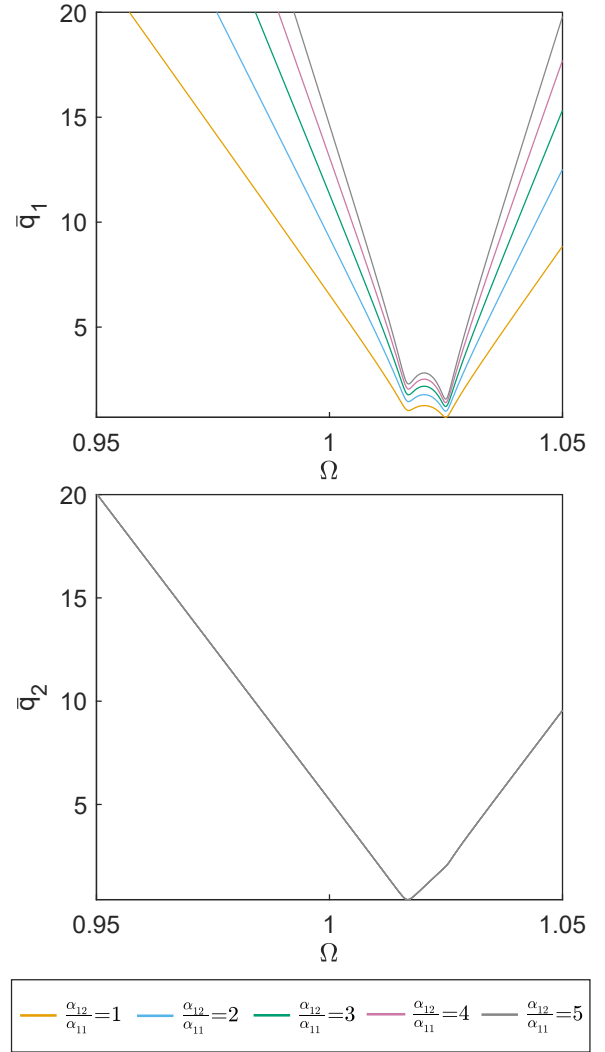
Fig. 23 The figures show the NS boundary behaviour corresponding to \omega_1 = 1 , \omega_2 = 2.005 , \mu_1 = \mu_2 = 1.5 \cdot 10^{-3} for different ratio \alpha_{12}/\alpha_{11} keeping \alpha_{12} = 5 \cdot 10^{-2} .
