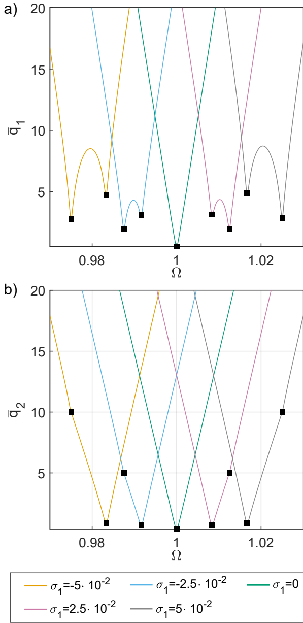
Fig. 9 Behaviour of the NS boundary curve when the detuning \sigma_1 = \omega_2 - 2\omega_1 is changed. The system parameter here considered are \alpha_{12} = 1 \cdot 10^{-2} , \alpha_{11} = 5 \cdot 10^{-3} , \mu_1 = \mu_2 = 5 \cdot 10^{-3} . The square markers correspond to the minima predicted by the analytical expression given in Appendix E, namely \Omega = \omega_2/2 and \Omega = (\omega_1 + \omega_2)/3 .
