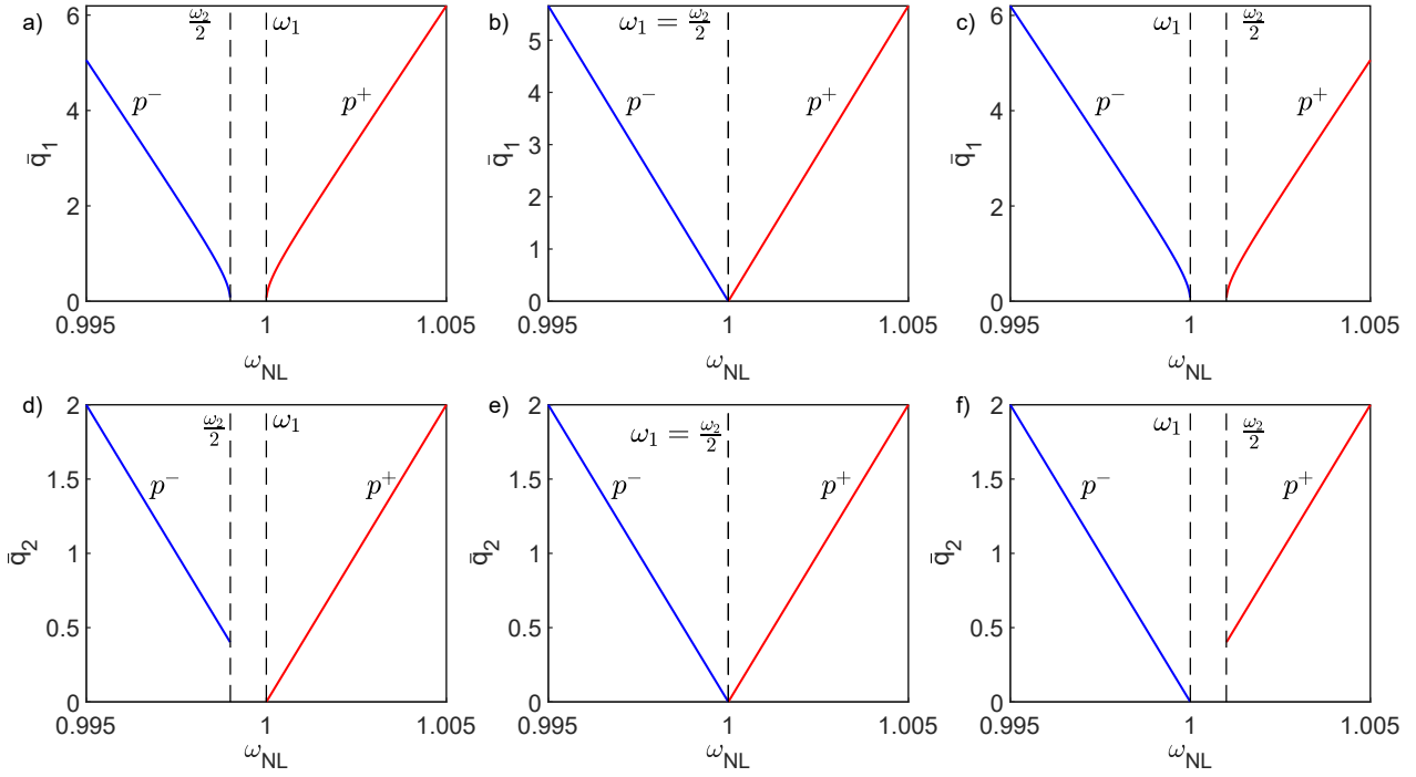
Fig. 3 Backbone curves of the two families p^+ (red curves) and p^- -modes (blue curves), in the plane (\omega_{\text{NL}}, a_1) (first row) and (\omega_{\text{NL}}, a_2) (second row), and for three different possible cases. First column: \omega_2/2 < \omega_1 , second column: \omega_2/2 = \omega_1 , third column: \omega_2/2 > \omega_1 . In the figure, \omega_1 = 1 , \alpha_{12} = 1 \cdot 10^{-2} , \alpha_{11} = 5 \cdot 10^{-3} .
