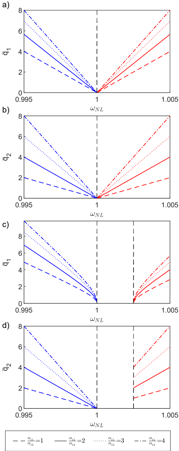
Fig. 22 Behaviour of the backbones when \alpha_{11}/\alpha_{12} is changed keeping fixed \alpha_{11} = 1 \cdot 10^{-2} . In these plots the line color marks with blue the p^- and with red the p^+ mode, the black dashed line marks \Omega = \omega_2/2 . Figs. a) and b) represent the backbone \bar{q}_1 and \bar{q}_2 respectively when \omega_2 - 2\omega_1 = 0 . Figs. c) and d) represent the backbone \bar{q}_2 and \bar{q}_2 respectively when \omega_2 - 2\omega_1 = 5 \cdot 10^{-3}
