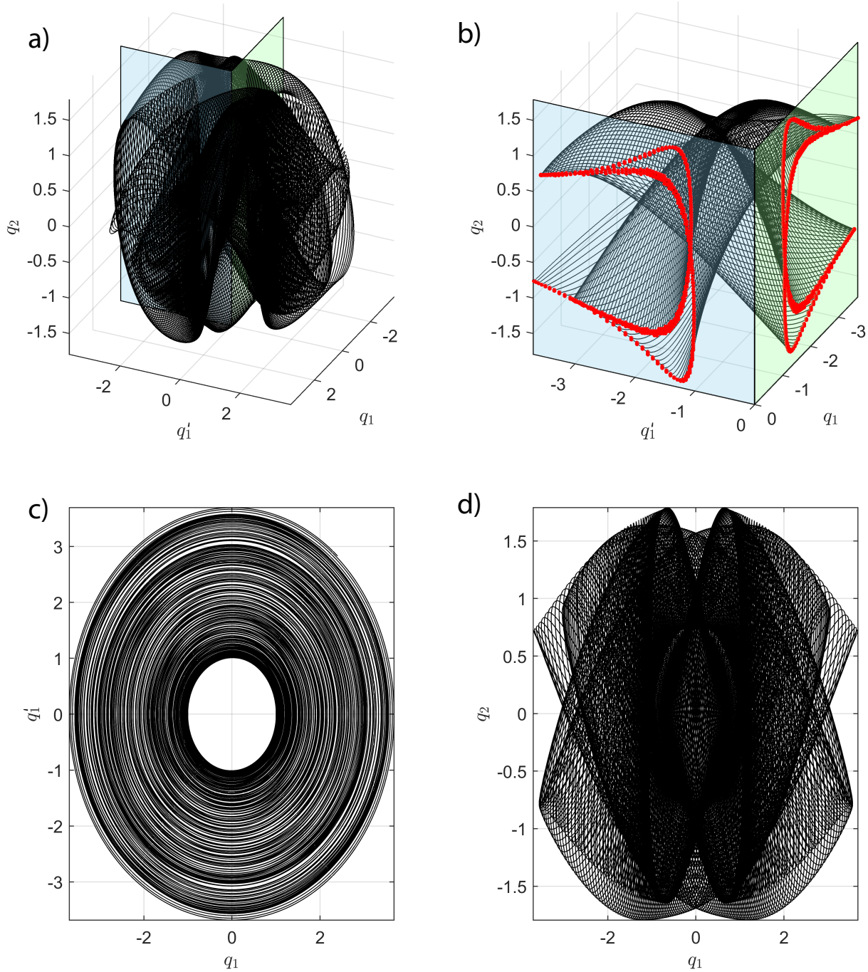
Fig. 16 Torus obtained by direct integration with RK4 algorithm of Eqs. (1) in the tuned case \omega_2 = 2\omega_1 . Only a short portion of the time history is plotted for sake of clarity
