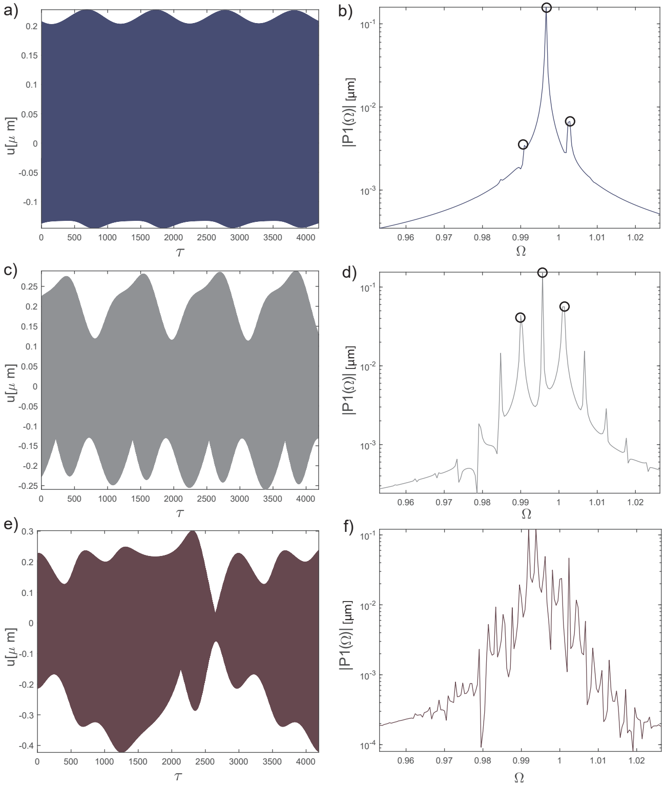
Fig. 20 Time histories (left column) and corresponding Frequency spectrum (right column) obtained by direct time integration of the full FE model, following the branch of QP solution by order of decreasing frequencies. First line: \Omega=0.9965 , birth of the QP solution. Second and third lines: \Omega= 0.9956 and 0.9939 .
