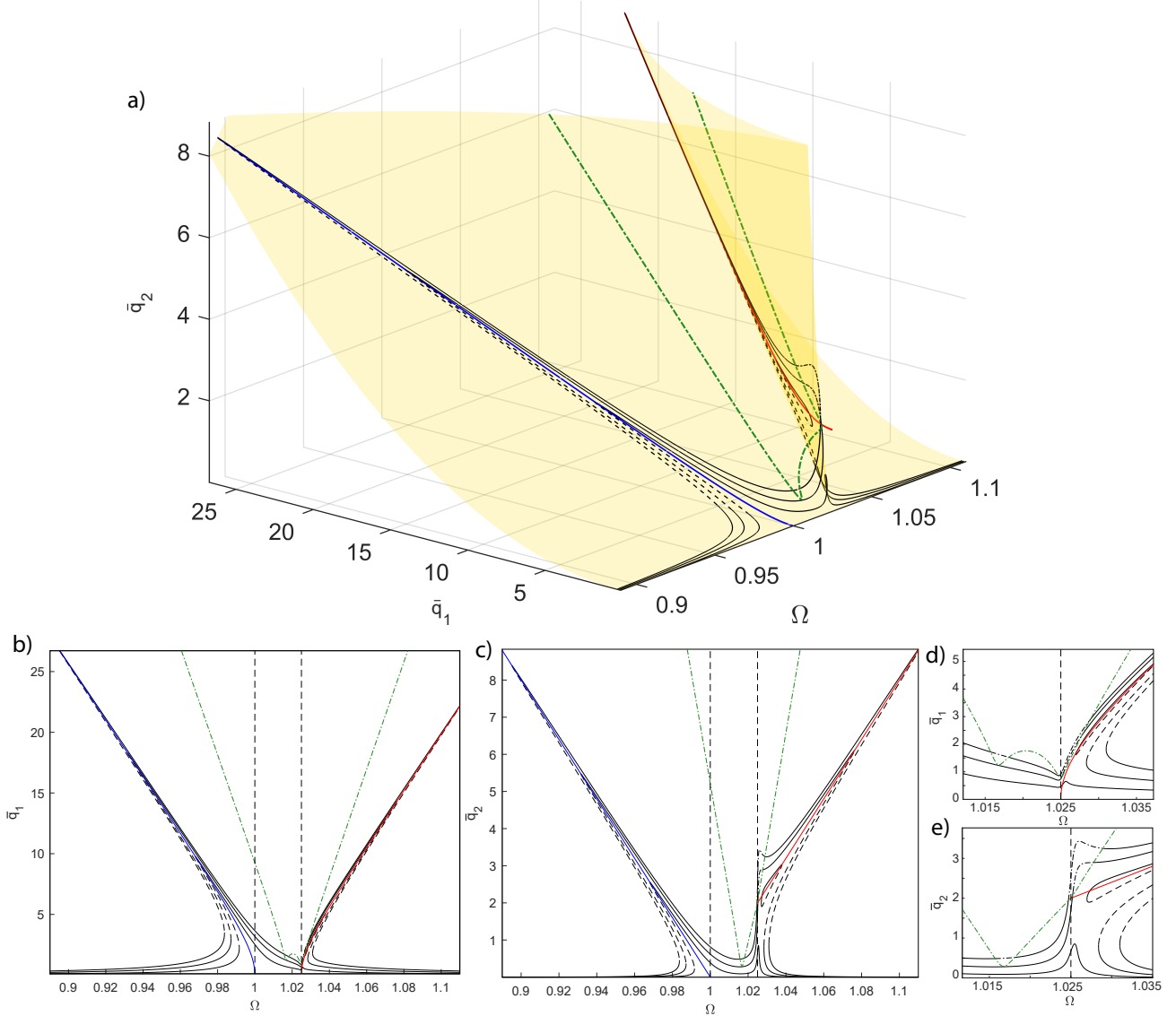
Fig. 7 FRF, backbone curves and NS boundary when \sigma_1 = 5 \cdot 10^{-2} , \mu_1 = \mu_2 = 1 \cdot 10^{-3} , \alpha_{12} = 5 \cdot 10^{-2} and \alpha_{11} = 2.5 \cdot 10^{-2} . The black continuous lines are the FRF (forced and damped solutions). The red and the blue lines are the backbones corresponding to the p^+ and p^- mode respectively. The black dashed line marks the \Omega = \omega_2/2 frequency. The green line is the NS boundary. In 3D figure in the space \Omega - \bar{q}_1 - \bar{q}_2 the orange surface is the manifold on which all the possible forced and damped solution lies and is given by Eq. (27b). Selected values of the forcing amplitude are F = 2.5 \cdot 10^{-2}, 5 \cdot 10^{-2}, 7.5 \cdot 10^{-2}
