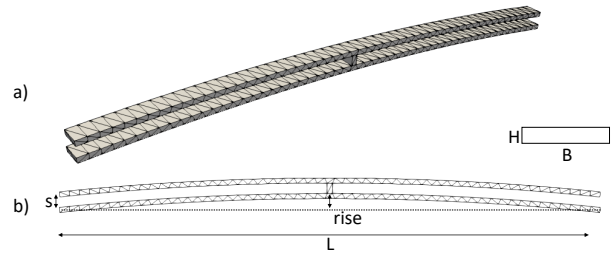
Fig. 12 a) 3D view of the FEM model used for the arch, b) scheme of the geometry of the shallow arch considered. B=20 \mu\text{m} , H=5 \mu\text{m} , L=530 \mu\text{m} , \text{rise}=13.4 \mu\text{m} , s=10 \mu\text{m} .
