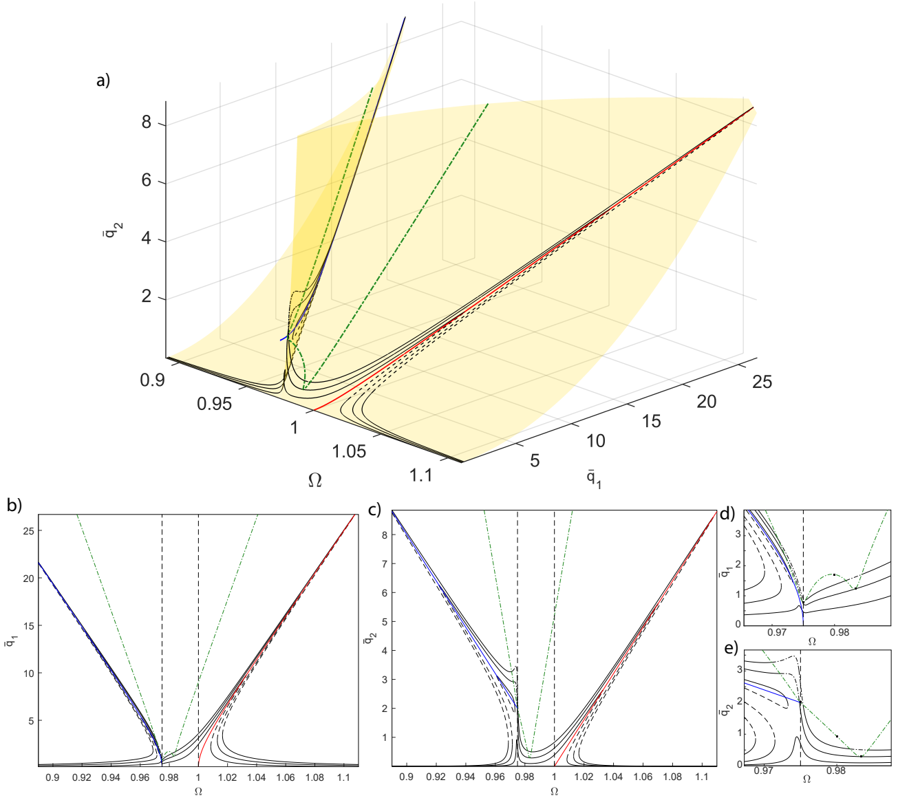
Fig. 8 FRF, backbone curves and NS boundary when \sigma_1 = -5 \cdot 10^{-2} , \mu_1 = \mu_2 = 1 \cdot 10^{-3} , \alpha_{12} = 5 \cdot 10^{-2} and \alpha_{11} = 2.5 \cdot 10^{-2} . The black continuous lines are the FRF (forced and damped solutions). The red and the blue lines are the backbones corresponding to the p^+ and p^- mode respectively. The black dashed line marks the \Omega = \omega_2/2 frequency. The green line is the NS boundary. In 3D figure in the space \Omega - \bar{q}_1 - \bar{q}_2 the orange surface is the manifold on which all the possible forced and damped solution lies and is given by Eq. (27b). Selected values of the forcing amplitude are F = 2.5 \cdot 10^{-4}, 5 \cdot 10^{-4}, 1 \cdot 10^{-3}
