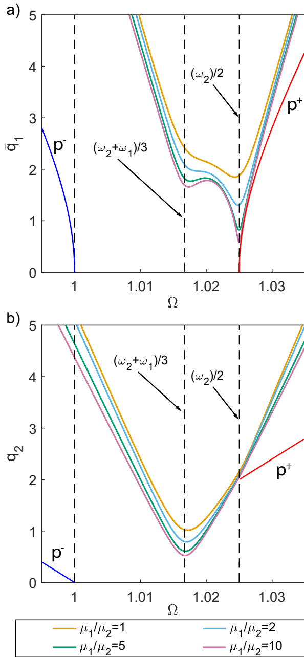
Fig. 11 Behaviour of the NS boundary curve, for \omega_1 = 1 , \omega_2 = 2.05 , \alpha_{12} = 5 \cdot 10^{-2} , \alpha_{11} = 2.5 \cdot 10^{-2} and different ratio \mu_1/\mu_2 keeping \mu_1 = 5 \cdot 10^{-3} fixed. The blue and red continuous lines are the backbone of the p^- and p^+ mode while the black dashed lines mark \Omega = \omega_2/2 and \Omega = (\omega_1 + \omega_2)/3 . The other lines corresponds to different damping levels as detailed in the legend.
