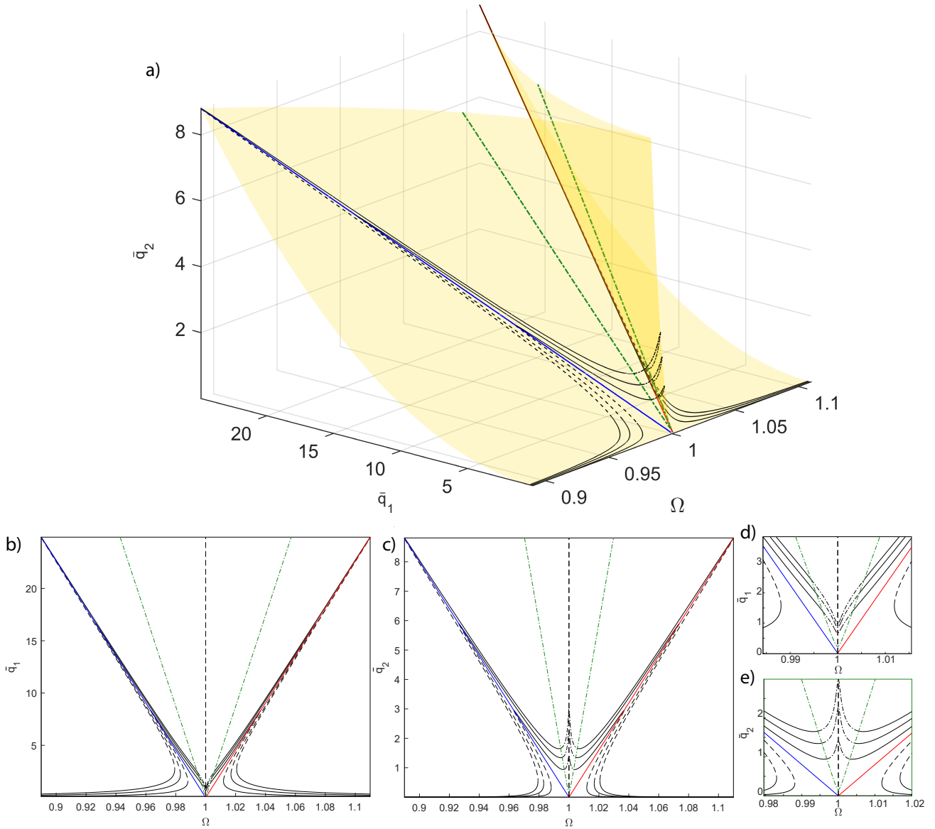
Fig. 6 FRF, backbone curves and NS boundary when \omega_1 = 1 , \omega_2 = 2\omega_1 , \mu_1 = \mu_2 = 1 \cdot 10^{-3} , \alpha_{12} = 5 \cdot 10^{-2} and \alpha_{11} = 2.5 \cdot 10^{-2} . The black continuous lines are the FRF (forced and damped solutions). The red and the blue lines are the backbones corresponding to the p^+ and p^- mode respectively. The black dashed line marks the \Omega = \omega_2/2 frequency. The green dash-dotted line is the NS boundary. In 3D figure in the space \Omega - a_1 - a_2 the orange surface is the manifold on which all the possible forced and damped solution lies and is given by Eq. (27b). Selected values of the forcing amplitude are F = 2.5 \cdot 10^{-2}, 5 \cdot 10^{-2}, 7.5 \cdot 10^{-2}
