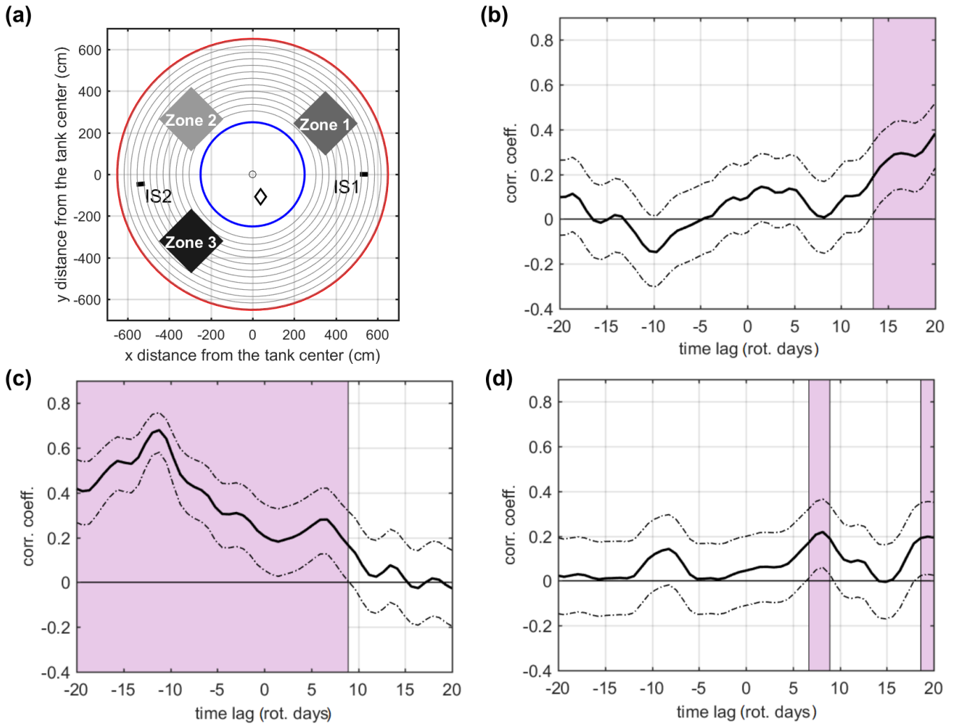
455 Figure 10: Vorticity correlations over the slope for EXP24. Position of the three selected zones (a); time-lagged correlation coefficients (solid line) between zones 1 and 2 (b), between zones 1 and 3 (c); between zones 2 and 3 (d). Upper and lower limits of the coefficients, corresponding to the 95% confidence level, are indicated by dashed-dot lines. Rose shaded areas indicate a positive correlation at 95% confidence limits. The limits for the maximum time lag were set by the calculated correlation time for the entire slope area, equal to approximately 22 rotation days.
