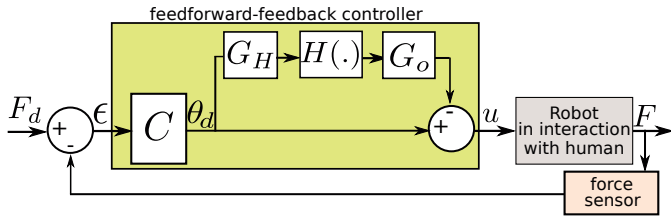
Fig. 7. Implementation diagram.
