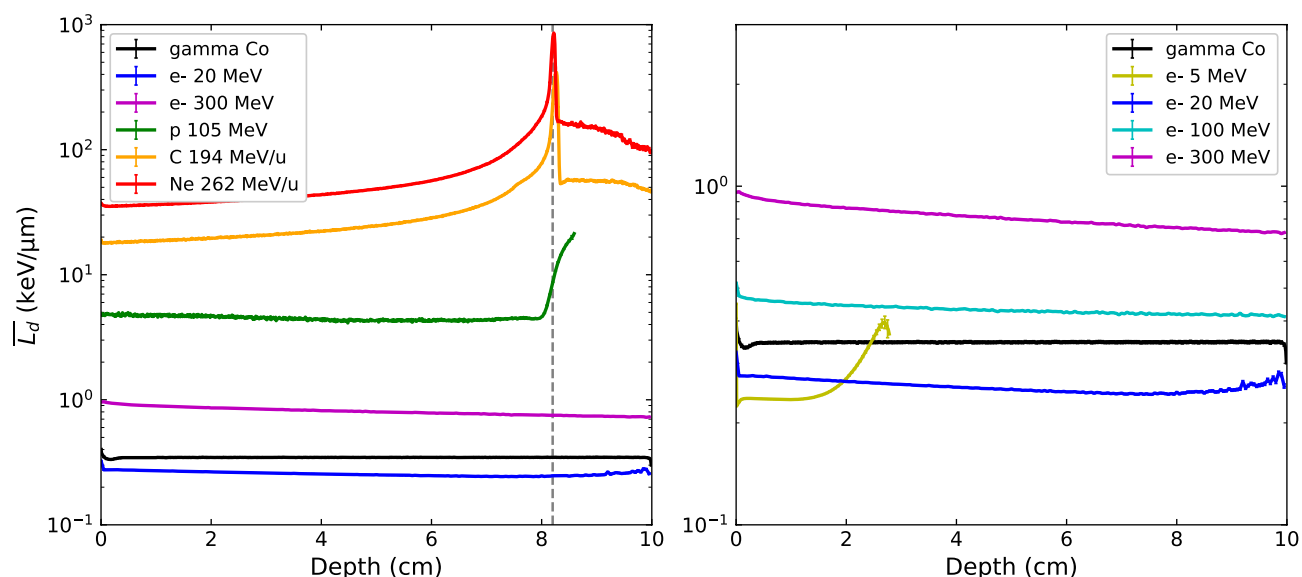
Figure 3. Dose-averaged LET profiles in depth to water for photon, clinical electrons, VHEE and ion beams (left), and details of the \overline{L}_d results for all electron beam energies (right). The vertical grey dashed line marks the Bragg peak position. \overline{L}_d values associated to doses lower than 0.1% of max dose are not shown to keep statistical relevance. Uncertainties on \overline{L}_d values in central axis voxels are less than 2%.
