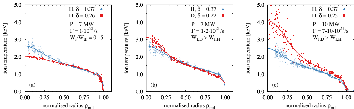
FIG. 9: Ion temperature profiles for H and D discharge pairs with matched pedestal top density. Low gas and low heating with matched W_{\text{fast}}/W_{\text{th}} (ID 5, 8) (a), matched toroidal rotation (ID 5, 1) (b) and high gas and high heating (ID 3, 7) (c).
