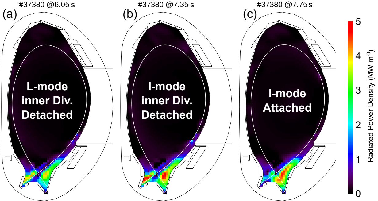
FIG. 5: Tomographic reconstruction of radiation measured by foil bolometers for L-mode with detached inner divertor (a), I-mode with detached inner divertor (b) and attached I-mode (c). The radiation present at the inner divertor leg disappears as the plasma re-attaches. No X-point radiator is observed.
