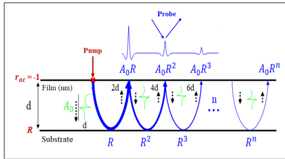
Figure 1: schematic diagram of the experiment and pulses in the material
