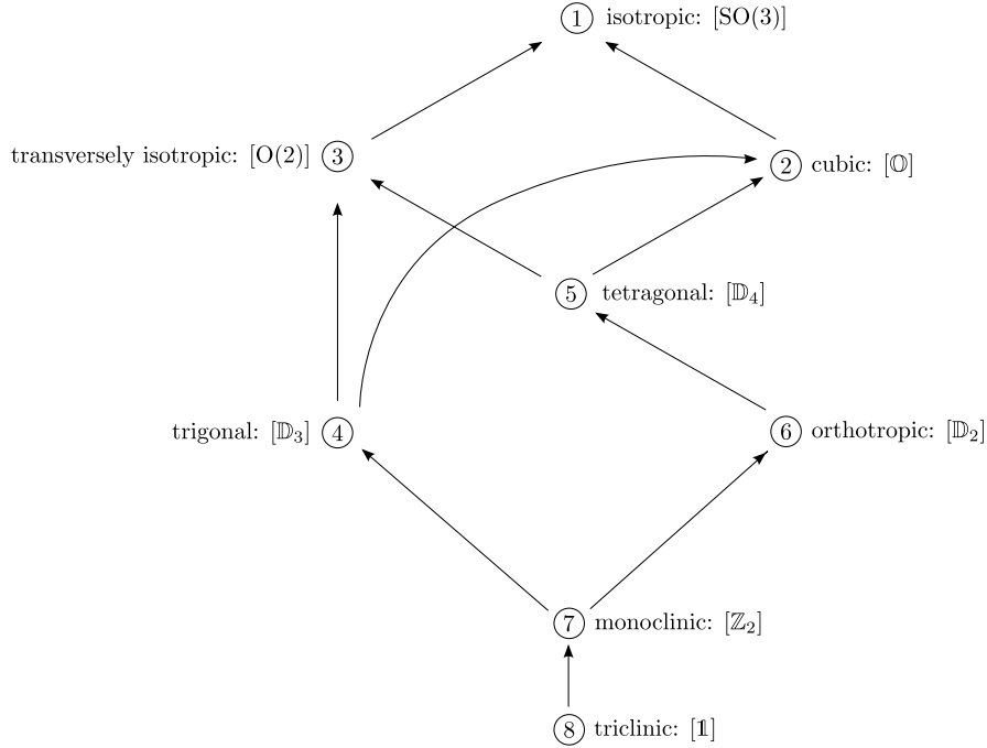
FIGURE 1. Symmetry classes of elasticity tensors and of fourth-order harmonic tensors [20, 17] (figure from [3]).
