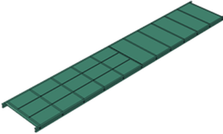
FIGURE 2: Smart composite platform CAD model [7].
