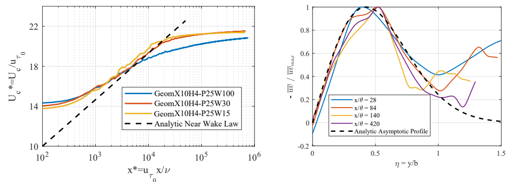
Figure 7. Comparison of the wake characteristics with empirical models in the near wake region (left) and the intermediate wake region ((right), for the computation GeomX10H4-P25W30, at different streamwise positions x/\theta ).
