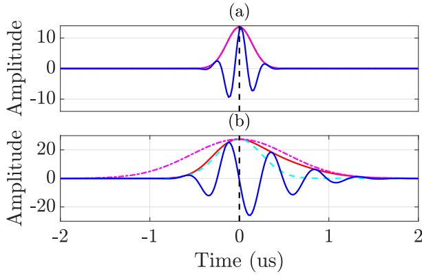
Figure 5: Ultrasonic waveform estimated from the SDH located at 20 mm depth with 3 MHz probe (-), asymmetric Gaussian envelope of the estimated ultrasonic waveform (- -), symmetric Gaussian envelope for the left part \alpha(1+r) (- - -), symmetric Gaussian envelope for the right part \alpha(1-r) (- - -).
