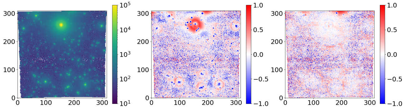
Figure 8: Left : Image of NGC5139 obtained with MUSE NFM at 850nm. Middle: residual map after stars detection and PSF subtraction using a Moffat-Gauss model for describing the PSF. Right: Residual map obtained using the PSFAO19 model. The mean residual error is improved by a factor 3 thanks to the new model definition.
