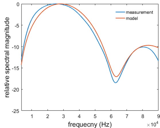
Figure 7: measured and calculated normalized frequency spectra of the filament's acoustic radiation at 25^\circ .
