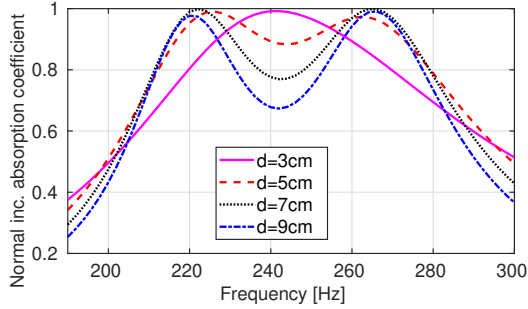
(b) Surfaces with the unit cell composed of 2 different types of resonators.
