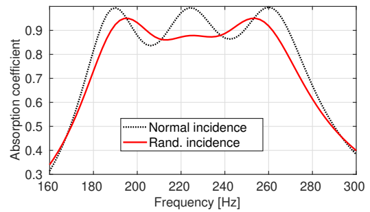
(c) Surface with the unit cell composed of 3 different types of resonators with dimensions as shown in Table 1, and a distance between the center of 2 adjacent resonators of 5 cm.
