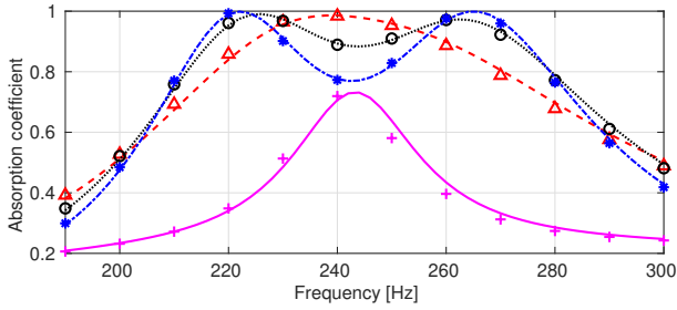
(b) Surface with the unit cell composed of 2 different types of resonators.
