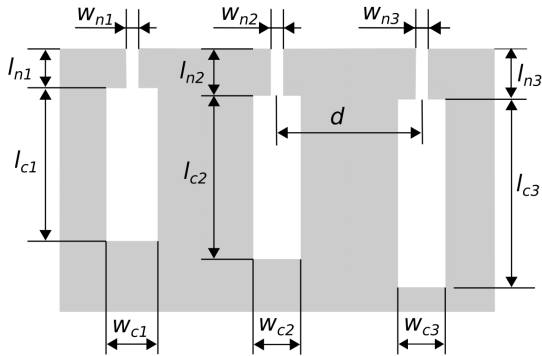
Figure 1: Schematic representation of the unit cell of a surface composed of a periodic arrangement of 3 different 2D Helmholtz resonators.
