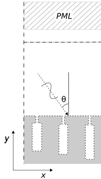
Figure 2: Sketch of the model used for the present study. The case shown corresponds to a surface with 3 resonators tuned to different frequencies. The boundaries identified with the dashed and dotted line, correspond to the boundaries to which a periodic and boundary layer impedance boundary condition was assigned respectively. And, the dotted dashed line identifies the line used for the estimation of the incident and reflected sound power according to Eq. 10. For ease of visualization, the dimensions shown here are not in scale with the dimensions of the model.
