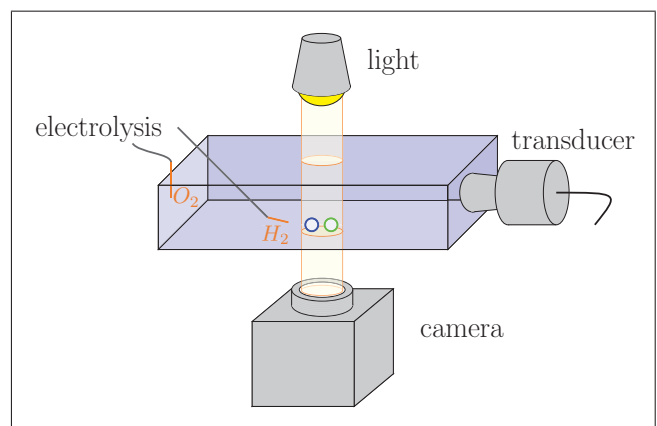
Figure 1. Schematics of the experimental setup.
