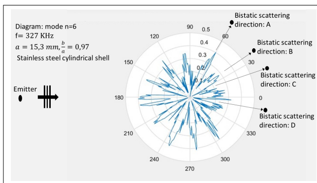
Figure 3. Angular diagram for f = 327\text{KHz} and vibration mode n=6
