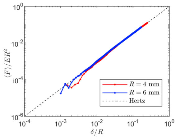
Figure 4. Numerical results: force F as function of displacement \delta .
