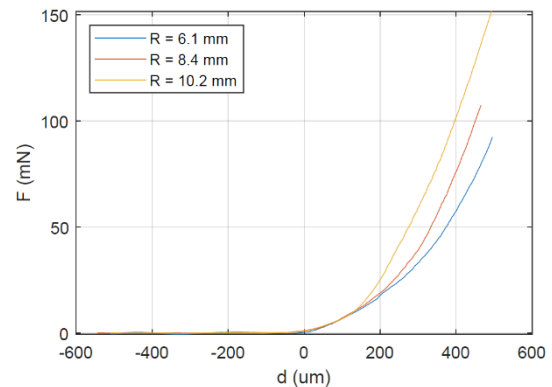
Figure 2. Force as function of displacement for 3 half spheres of different radius.
