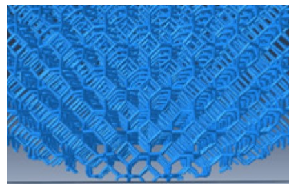
Figure 3. Detail of the model at the contact point between the rigid plane and the half sphere modeled by Kelvin cells.
