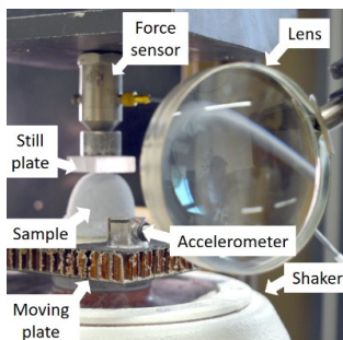
Figure 1. Experimental set-up for quasistatic measurement of the contact force of a melamine half sphere sample.
