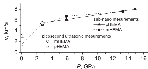
Fig. 3 The summary of results for the evaluation of longitudinal sound velocity using subnanosecond ultrasonic technique: solid circles – mHEMA; solid triangles – pHEMA. Using picosecond ultrasonic measurements: open circles – mHEMA; open triangles – pHEMA.
