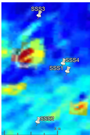
Figure 10. Positions of a same object in the different SSS mosaics, plotted on the DTM standard deviation map. The considered object is the red disk on the left.
