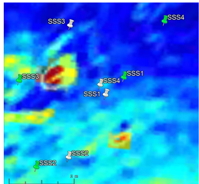
Figure 11. Positions of a same object in the SSS mosaics, plotted on the DTM standard deviation map. The considered object is the red circle on the left. White marks, use of FLS tracking, green marks, use of a layback of 10 m.
