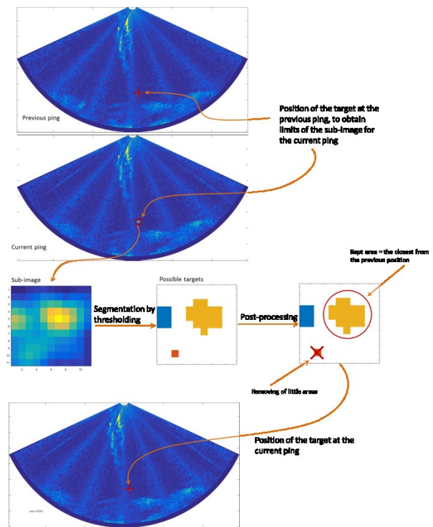
Figure 4. Schematic of the tracking process.
