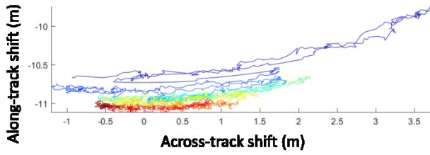
Figure 5. Tracked SSS positions in the FLS image. Positions are here presented in the FLS baseline (positive across-track values at starboard and negative along-track values behind the FLS). Colors are representing time passing (blue for the first pings to red for the last pings)
