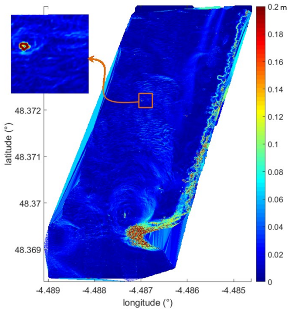
Figure 9. local standard deviation of the DTM: little objects can be easily detected.
