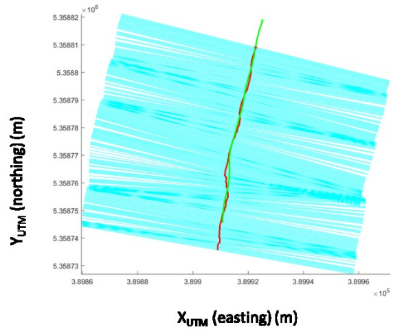
Figure 6. Example of SSS trajectory (in red) comparing to the ship trajectory (in green). Cyan lines represent SSS range at each ping (lines are not parallel due to the heading)
