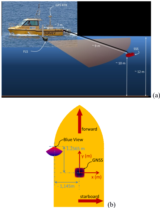
Figure 1. (a) Experimental protocol to track the SSS with a FLS. (b) Sonar position relative to the GNSS.
