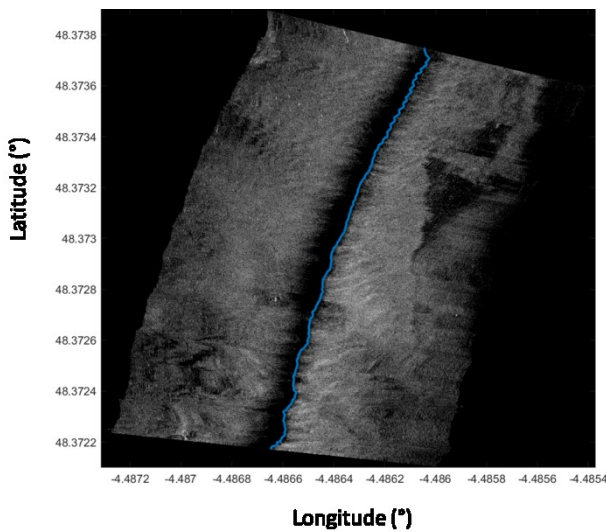
Figure 7. Example of SSS mosaic
