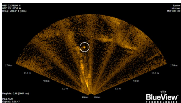
Figure 3. Example of image showing the SSS signature in the FLS data (surrounded by white)
