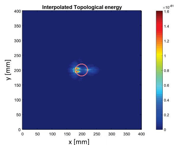
Figure 4. Topological energy for a flat-bottomed hole of diameter d=20\text{mm} and depth p=H/4=1.25\text{mm}
