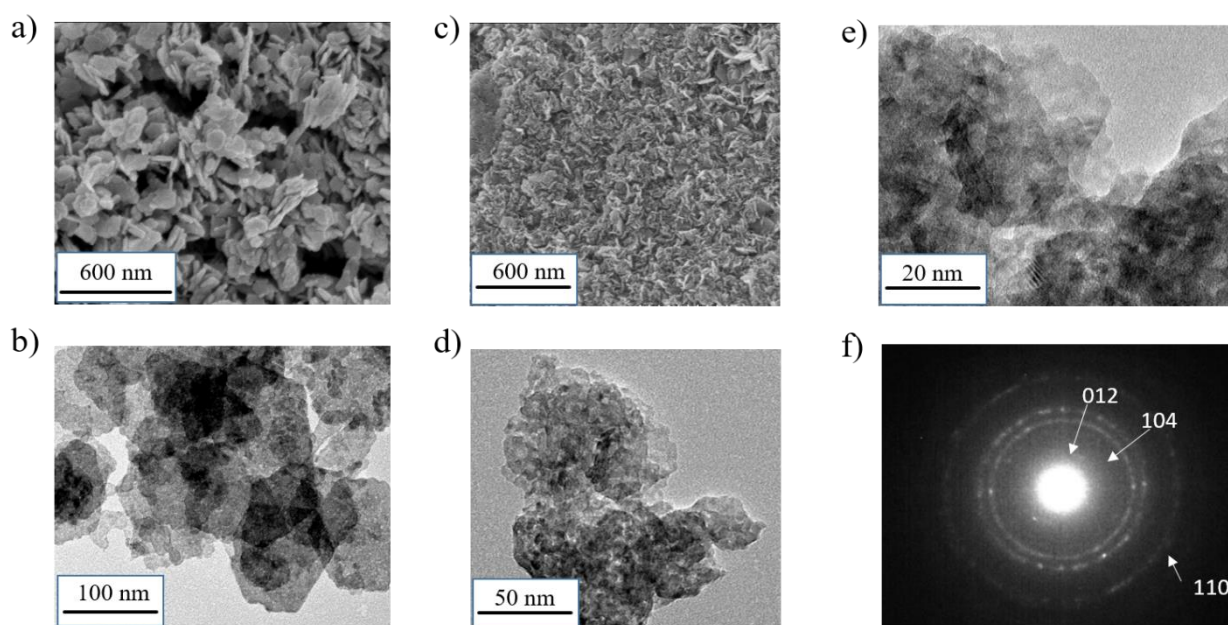
Figure 2. (a) SEM images of \beta 3-pH 14 ; (b) TEM images of \beta 3-pH 14 ; (c) SEM images of \beta 3-pH γ ; (d,e) TEM images of \beta 3-pH γ ; (f) electron diffraction of \beta 3-pH γ .
