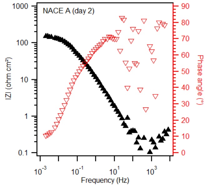
FIGURE 4: EIS diagram (Bode / Phase angle plot) of X65 membrane after 2 days exposure, without O 2 contamination, in NACE A buffer solutions held at T = 24°C under 100 kPa H 2 S.
