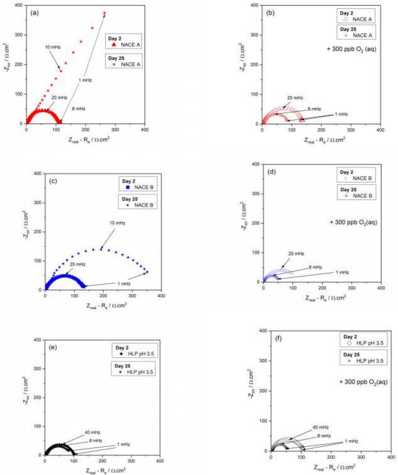
FIGURE 3: EIS diagrams of X65 membrane at various exposure times of after 2 days and 25 days of exposure, without and with O 2 contamination ( [O_2]_{aq} = 300 ppb) in (a-b) NACE A (c-d) NACE B and (e-f) HLP pH 3.5 buffer solutions held at T = 24^\circ\text{C} under 100 kPa H 2 S.
