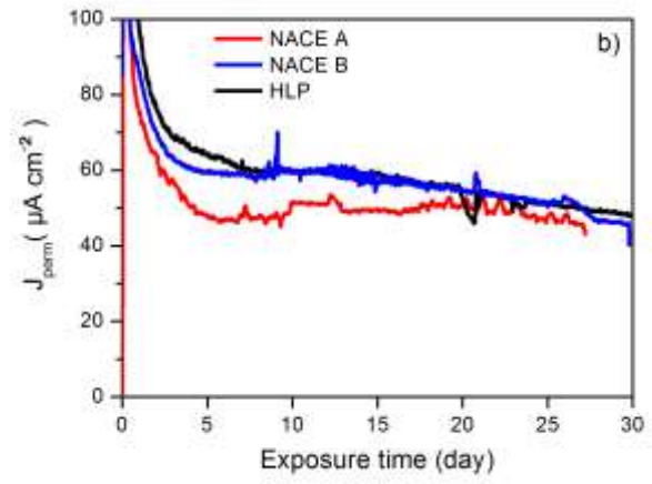
FIGURE 7: Hydrogen permeation across X65 membrane exposed to buffer solutions at T = 24^{\circ}\text{C} under 100 kPa \text{H}_2\text{S} (a) without and (b) with deliberate \text{O}_2 contamination ( [\text{O}_2]_{\text{aq}} = 300 ppb).
