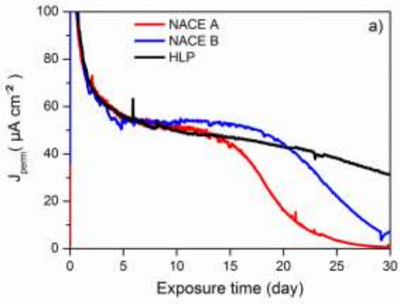
FIGURE 7: Hydrogen permeation across X65 membrane exposed to buffer solutions at T = 24^{\circ}\text{C} under 100 kPa \text{H}_2\text{S} (a) without and (b) with deliberate \text{O}_2 contamination ( [\text{O}_2]_{\text{aq}} = 300 ppb).
