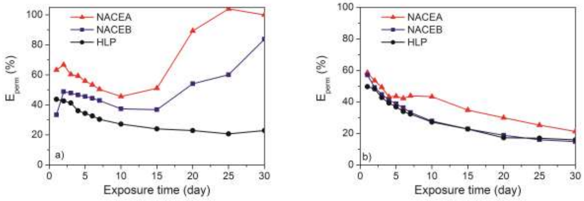
FIGURE 8: Permeation efficiencies across X65 membrane exposed to buffer solutions at T = 24^{\circ}\text{C} under 100 kPa H 2 S (a) without and (b) with deliberate O 2 contamination ( [\text{O}_2]_{\text{aq}}=300 ppb).
